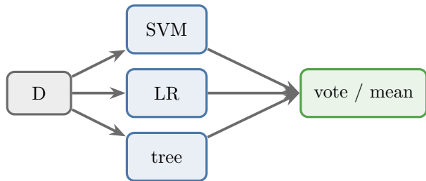
(a) voting
