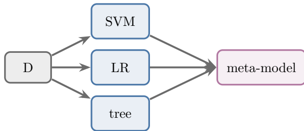
(b) stacking
