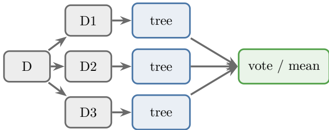
(c) bagging
