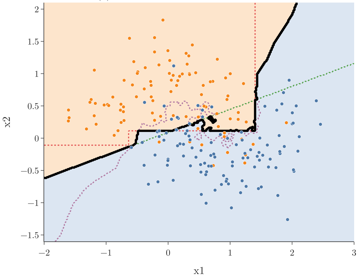
(a) classification: three models and the vote
