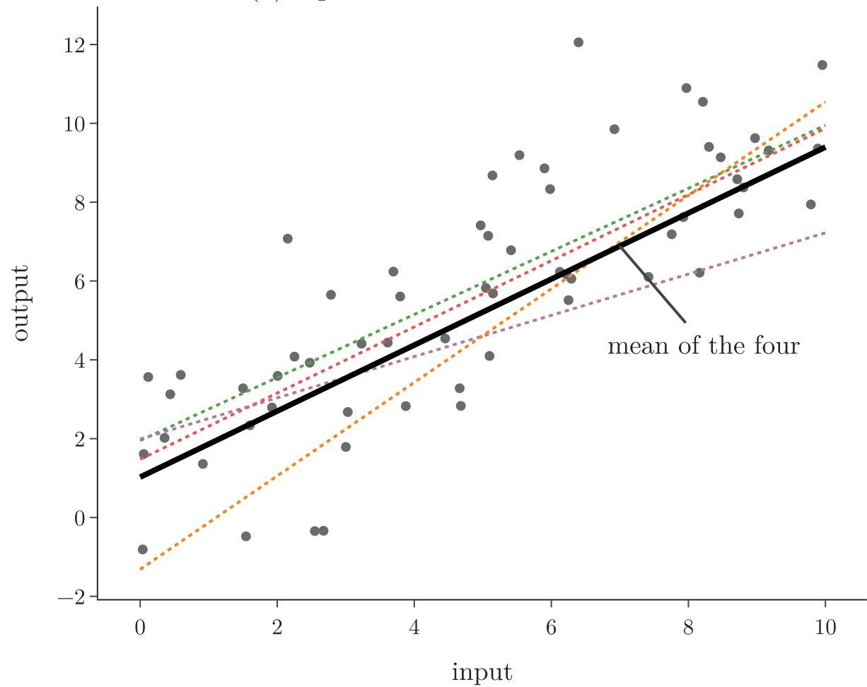
(b) regression: four lines and their mean
