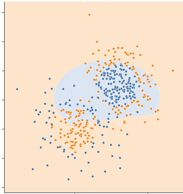
voting (hard): 0.63
