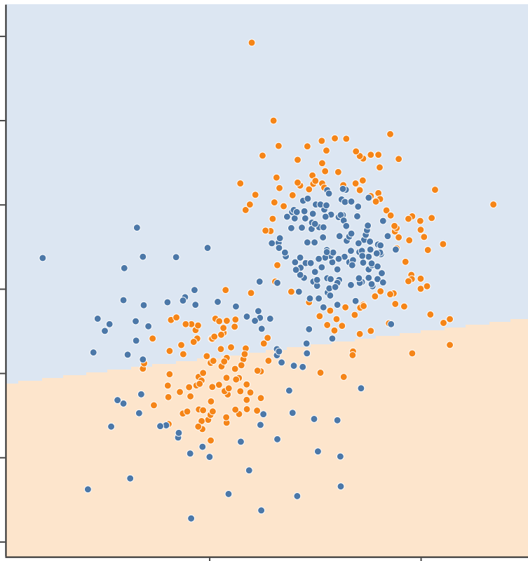
logistic regression: 0.53
