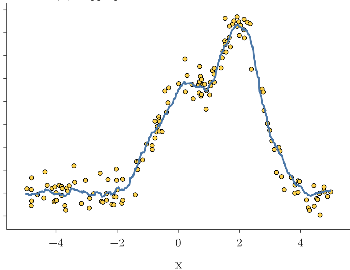
(b) bagging, 50 trees of 25 rows: test R^2 0.95
