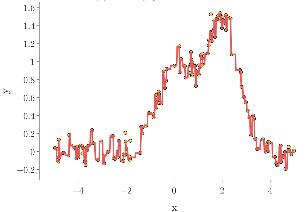
(a) one fully grown tree: test R^2 0.92
