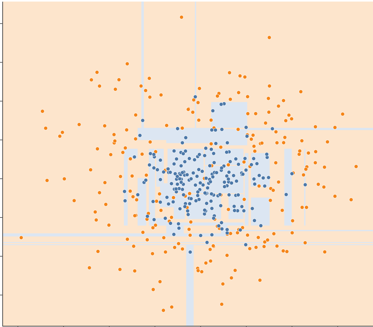
(a) one fully grown tree: train 1.00, test 0.86
