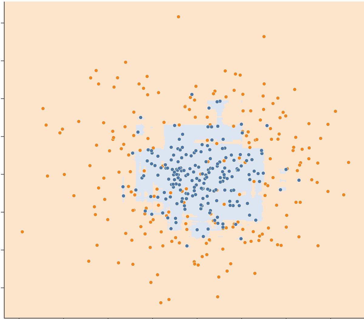
(b) random forest, 500 trees: train 1.00, test 0.91
