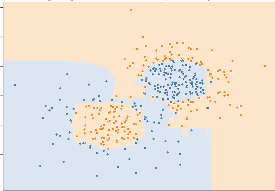
ccp_alpha = 0: 41.9 leaves, accuracy 0.887
