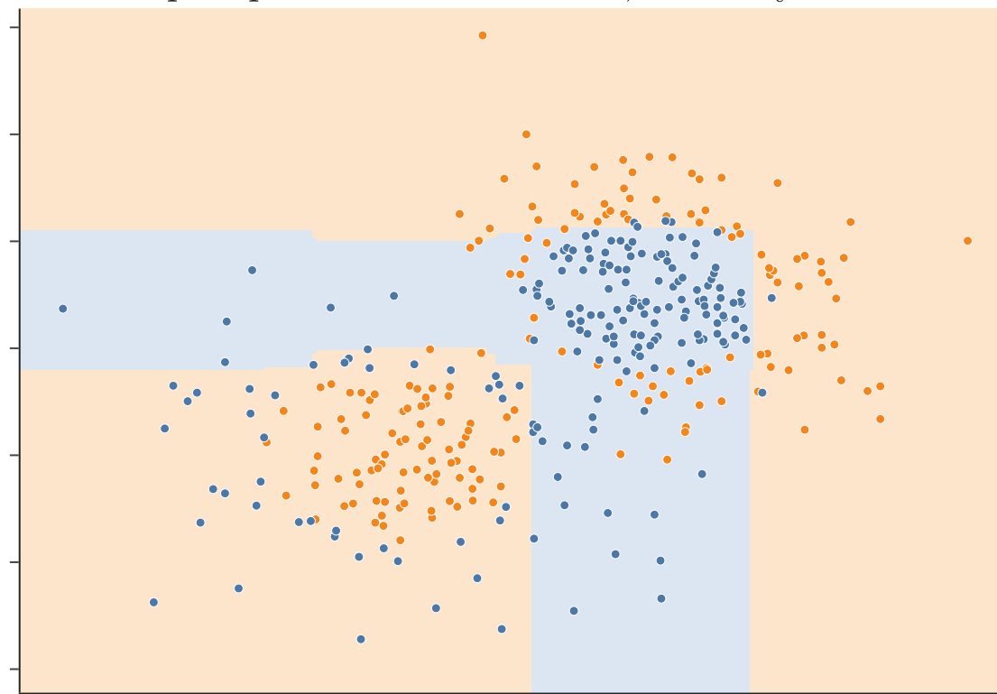
ccp_alpha = 0.05: 3.9 leaves, accuracy 0.776
