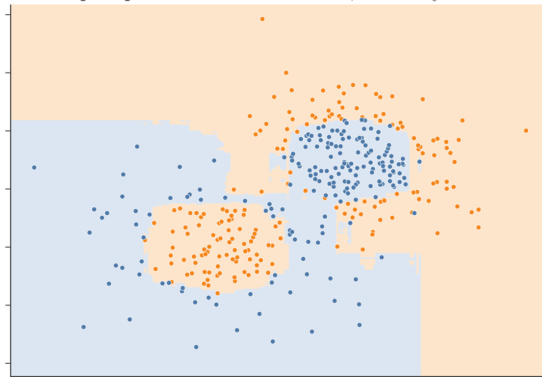
ccp_alpha = 0.002: 39.2 leaves, accuracy 0.886
