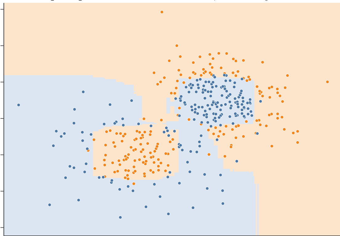
ccp_alpha = 0.01: 12.1 leaves, accuracy 0.878
