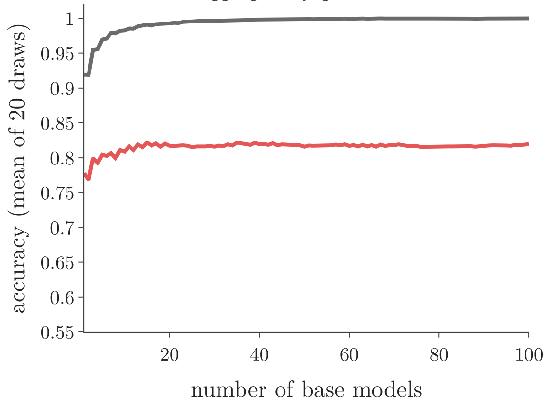
bagging: fully grown trees
