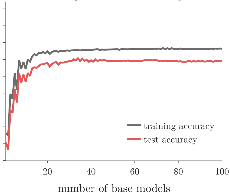
boosting: AdaBoost with stumps
