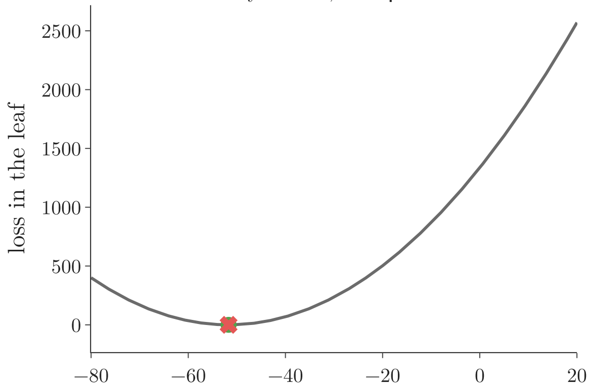
squared error tree says -51.70, best \gamma = -51.70
