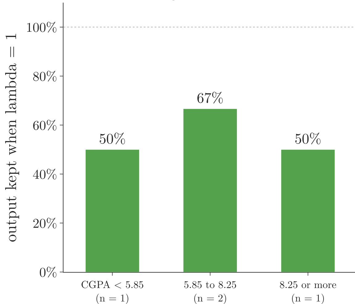
regression leaves
