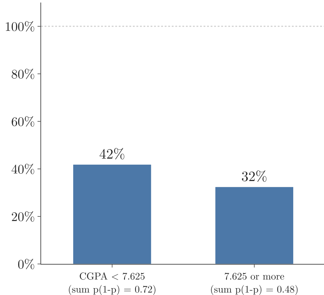
classification leaves
