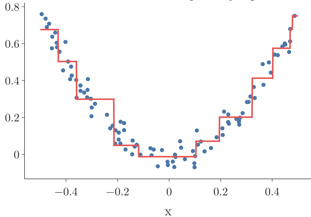
boosted trees: flat steps and jumps
