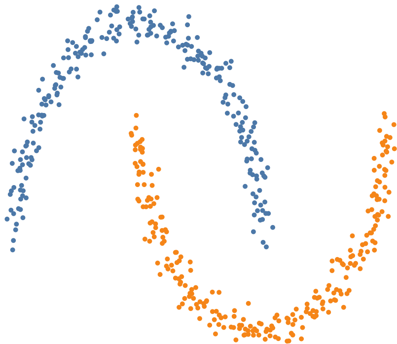
two moons
