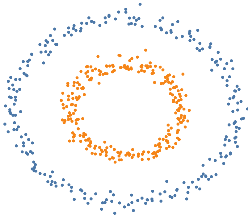
two circles
