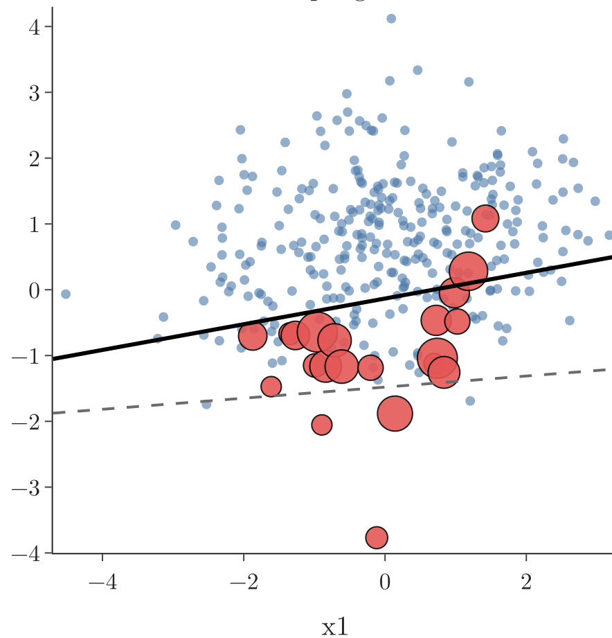
Random oversampling: 299 + 299 rows
