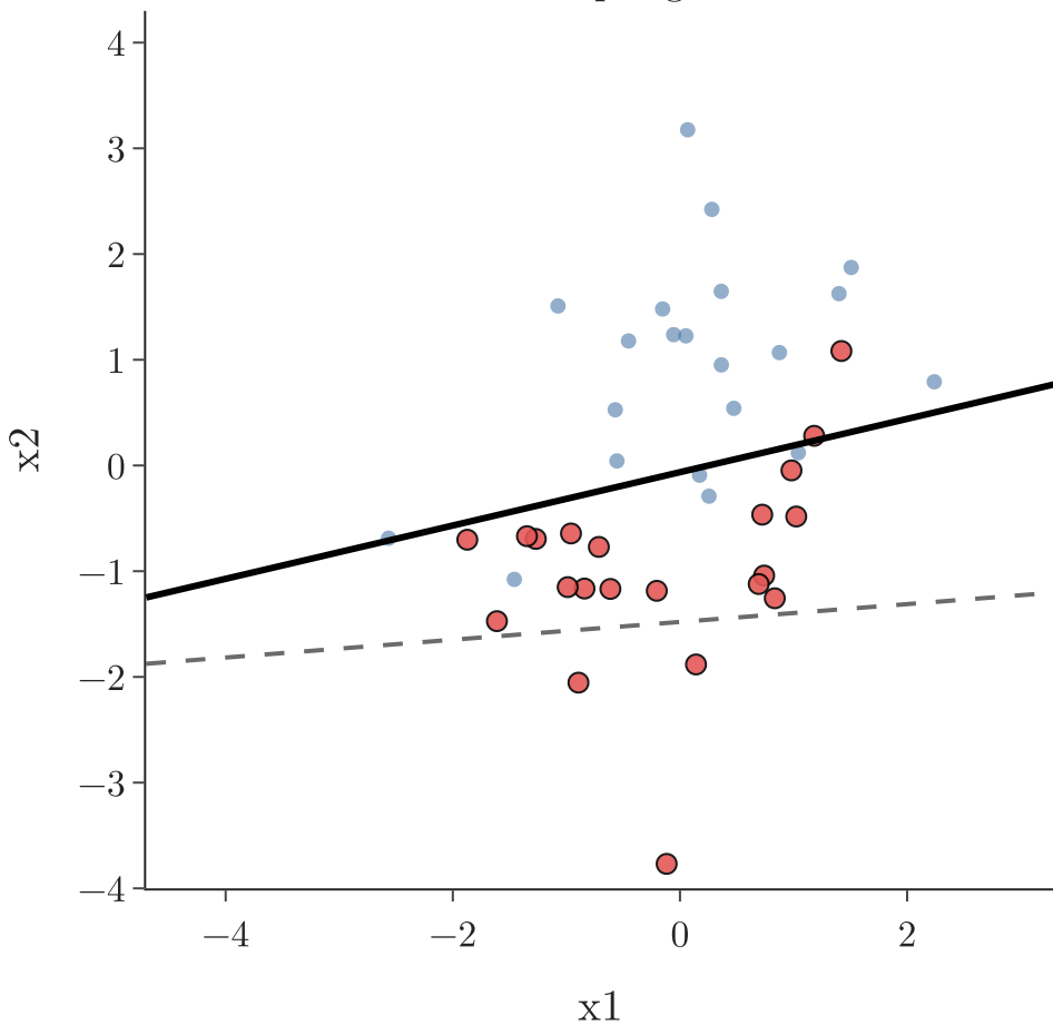
Random undersampling: 21 + 21 rows
