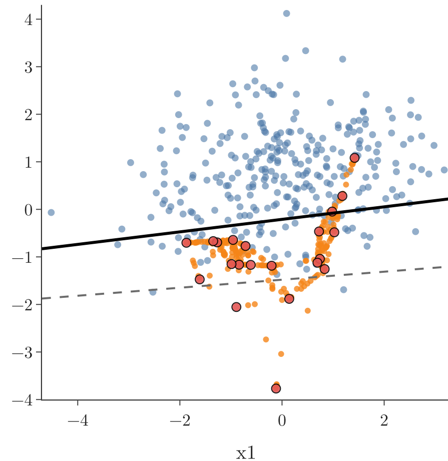
SMOTE: 299 + 21 + 278 new rows
