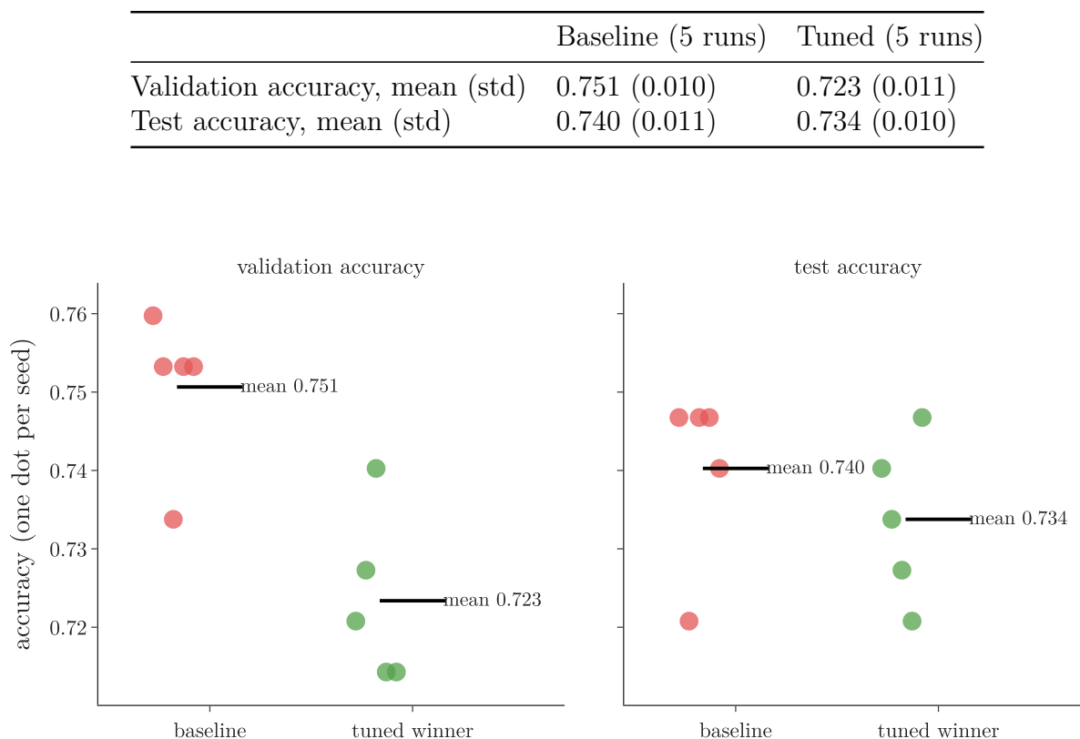
Figure 8: Pima diabetes: the baseline and the tuned winner, each retrained with 5 seeds. One dot per run; the black bar is the mean.
