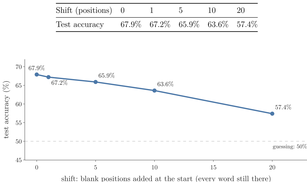
Figure 6: The same test reviews, pushed further to the right. Every word is still there, yet the accuracy falls towards guessing
