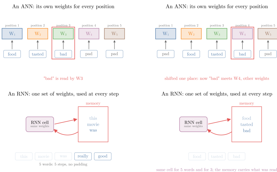
Figure 7: Top: an ANN gives each position its own weights, so when “food tasted bad” shifts one place, “bad” meets W_4 instead of W_3 . Bottom: an RNN reads one word at a time through one cell with the same weights and passes a memory on; the 5-word and the 3-word review use the same cell with no padding. The memory is drawn as the words read so far, older ones fainter; the next Note shows the numbers it really holds
