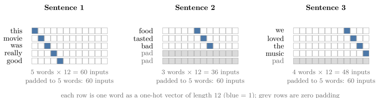
Figure 3: Each word becomes a one-hot row of length 12; a review becomes a stack of rows. Shorter reviews are padded with rows of zeros up to the longest one, 5 words
