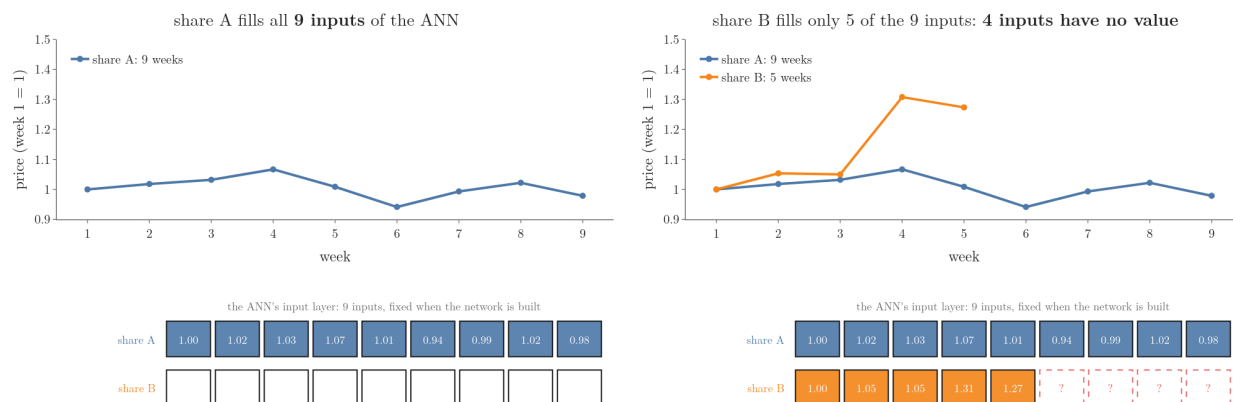
Figure 2: Real weekly prices of two shares in early 2018, each divided by its first price: 9 weeks of share A (Google), 5 weeks of share B (Netflix). An ANN’s input layer has a fixed number of inputs; the 9-week series fills it, the 5-week series leaves 4 inputs with no value (idea after StatQuest, “Recurrent Neural Networks (RNNs), Clearly Explained!!!”)
