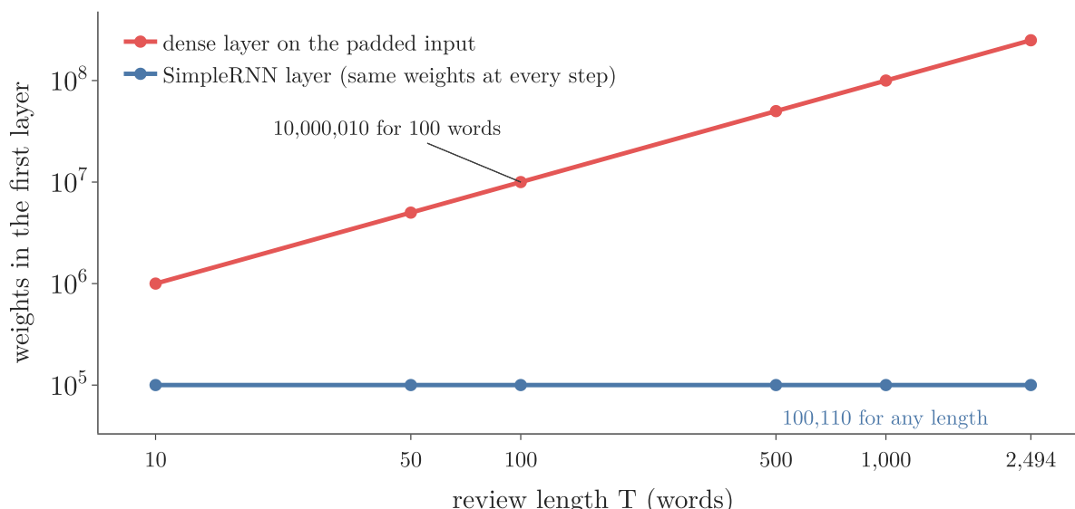
Figure 8: Weights in a first layer of 10 nodes over a 10,000-word vocabulary. The dense layer grows with every extra word (red); the RNN layer stays at 100,110 for any length (blue). Both axes are logarithmic
