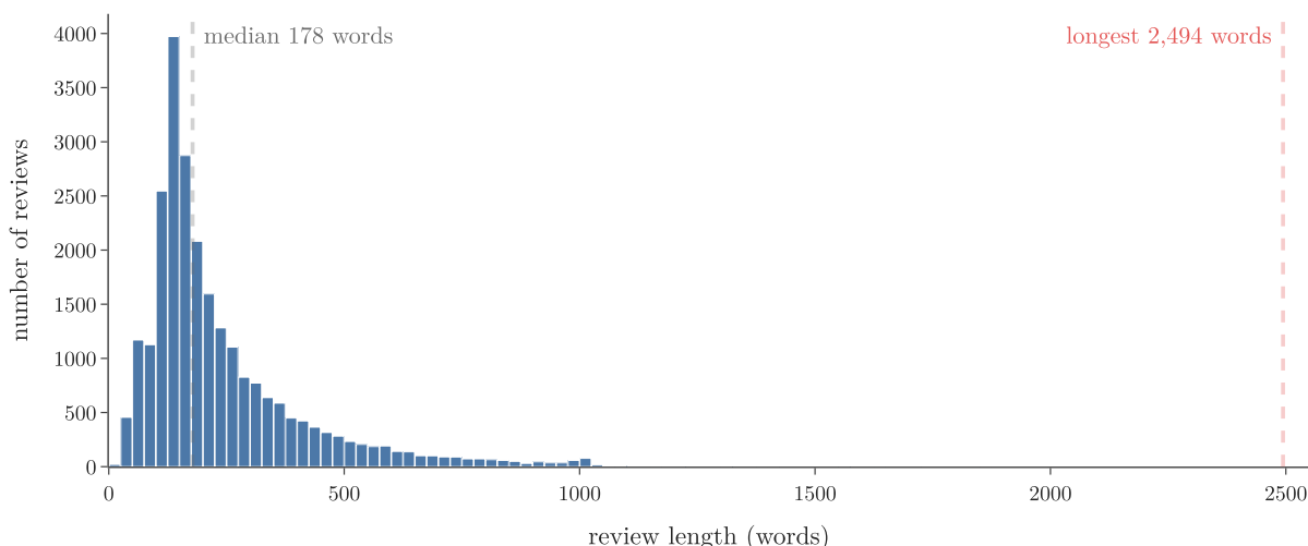
Figure 4: Lengths of the 25,000 IMDB training reviews. Most are a few hundred words long, but a long tail reaches 2,494 words
