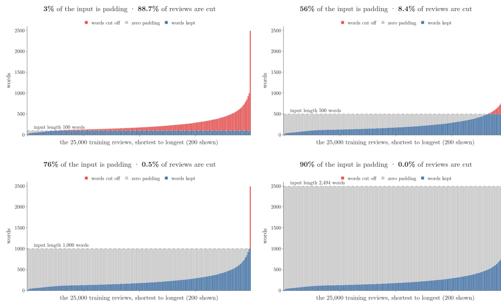
Figure 5: Every IMDB training review padded (grey) or cut (red) to one input length, from 100 to 2,494 words. A short length cuts most reviews; a length that cuts none makes 90% of the input zeros
