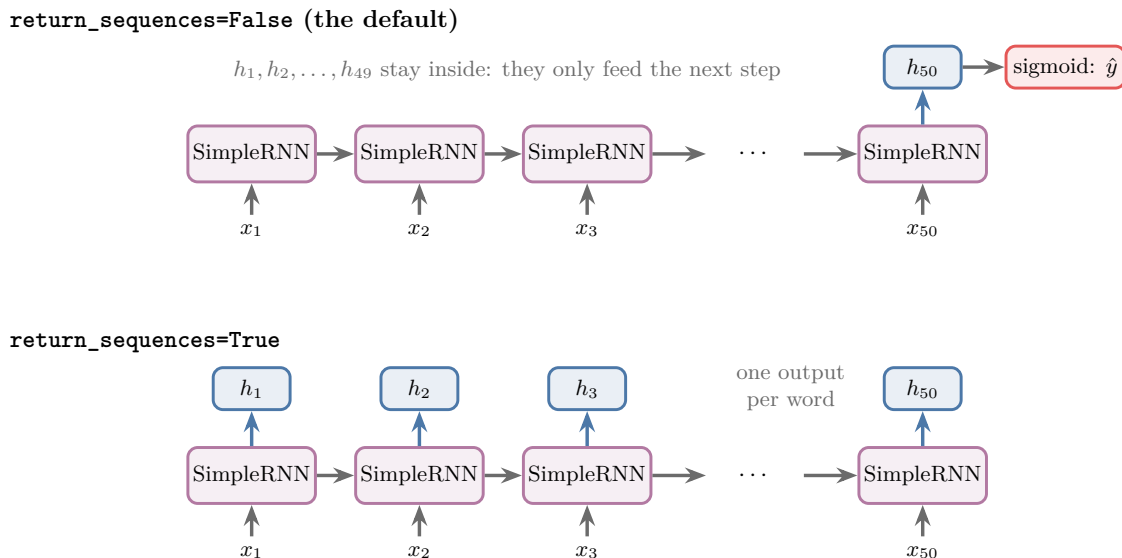
Figure 4: The SimpleRNN of section 5 unrolled over a review’s 50 integers. Top: with return_sequences=False only h_{50} goes on to the sigmoid output. Bottom: with True every hidden state leaves the layer, one per word
