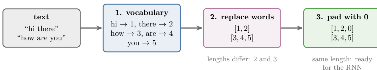
Figure 2: Integer encoding of two sentences: build the vocabulary and number its words, replace every word by its number, then pad the shorter sequence with 0
