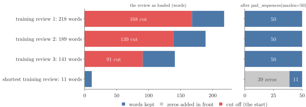
Figure 3: pad_sequences(maxlen=50) on four IMDB training reviews. The three long ones lose their start (red) and keep their last 50 words (blue); the shortest review, 11 words, gets 39 zeros in front
