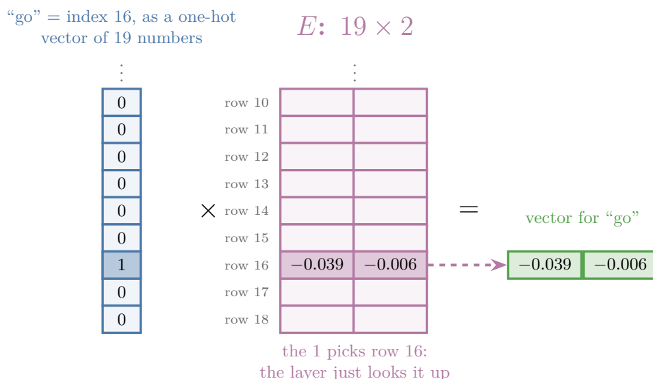
Figure 5: The embedding layer as a lookup: the one-hot vector of “go” (index 16) times E keeps row 16 of E , which becomes the word’s dense vector
