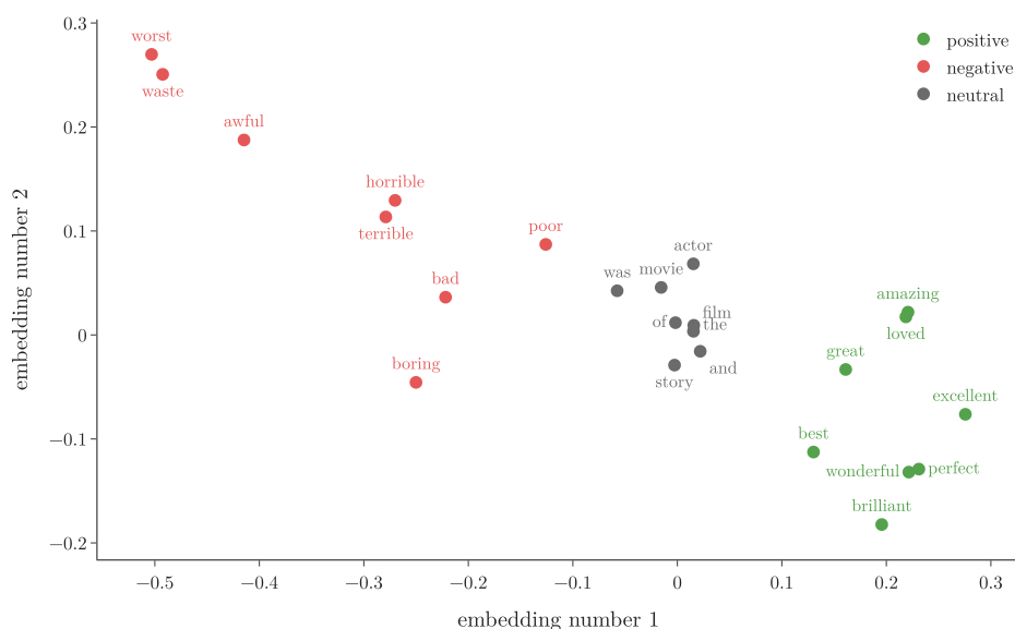
Figure 6: The learned 2-number vectors of a few IMDB words after training. Positive words (green) and negative words (red) end up on opposite sides; frequent neutral words (grey) sit between them
