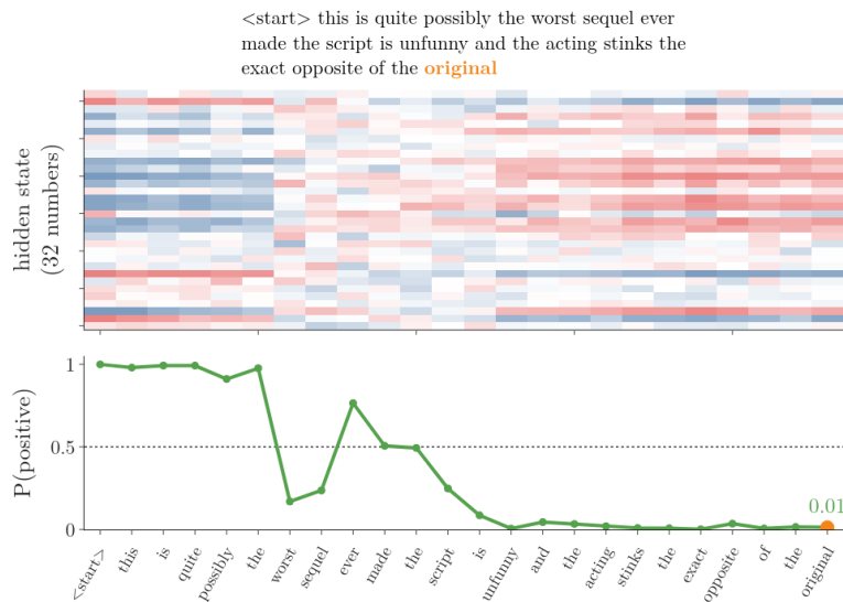
Figure 8: The trained embedding model reads a negative test review word by word. Top: the 32 numbers of the hidden state after each word (blue positive, red negative). Bottom: the prediction if the review stopped at that word. The prediction falls from 0.98 to 0.17 at “worst”, climbs back to 0.77 at “ever”, then falls for good and ends at 0.013
