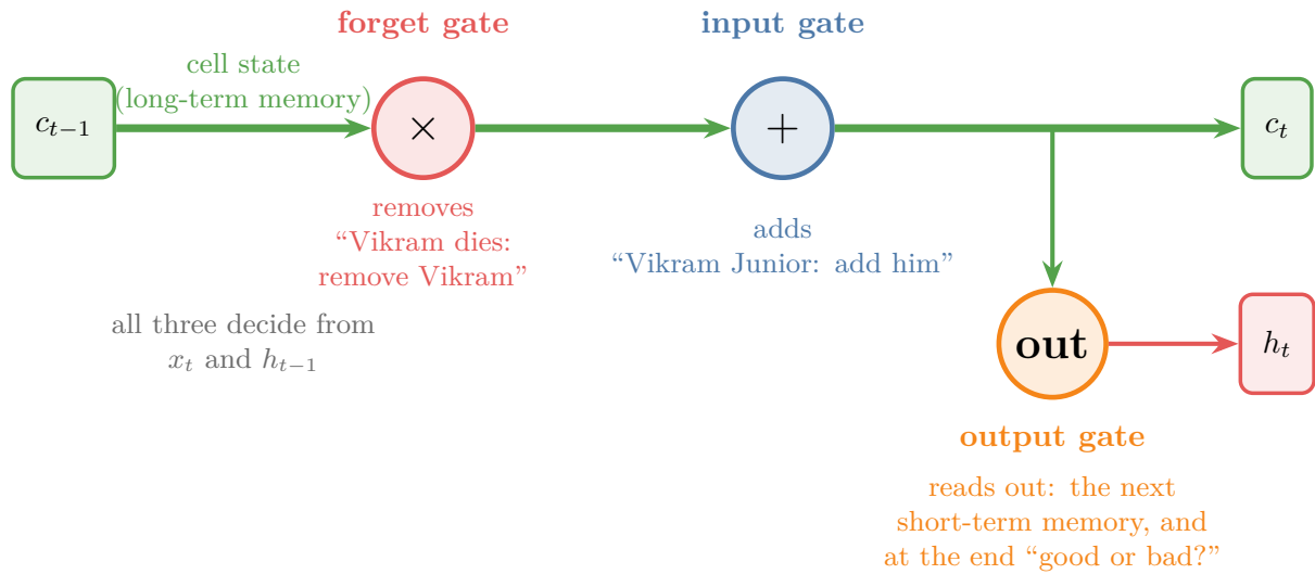
Figure 5: The three gates placed on the long-term memory. The forget gate multiplies the cell state (removes), the input gate adds to it, and the output gate reads from it to give h_t . The examples come from the story of section 4
