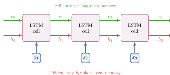
Figure 1: A simple RNN passes one hidden state from step to step. An LSTM passes two: the cell state (green, long-term memory) and the hidden state (red, short-term memory)
