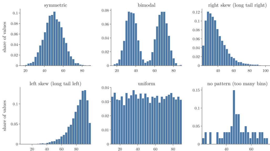
Figure 6: Six shapes a histogram can take
