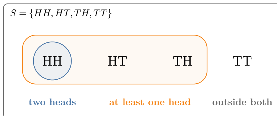
Figure 3: Tossing a coin twice: the sample space and two events
