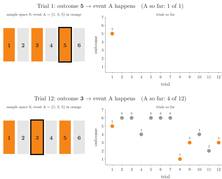
Figure 2: The random experiment “roll a die” run in 12 simulated trials. Left: the sample space, with the event A = \{1, 3, 5\} in orange and the current outcome boxed. Right: the outcome of every trial so far, orange when A happened.
