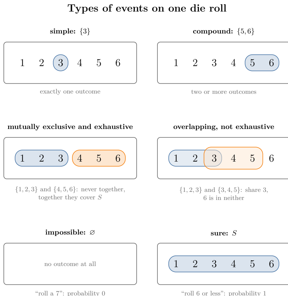
Figure 5: Types of events on one die roll
