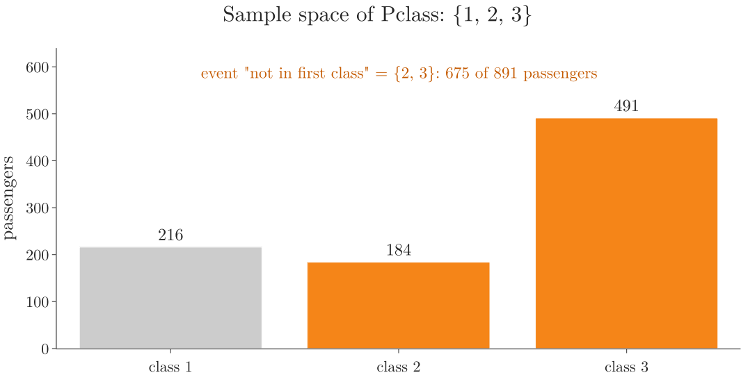
Figure 4: Each class of Pclass with its number of passengers; together the classes form the sample space \{1, 2, 3\} . The event “not in first class” = \{2, 3\} (orange) covers 675 of the 891 passengers.
