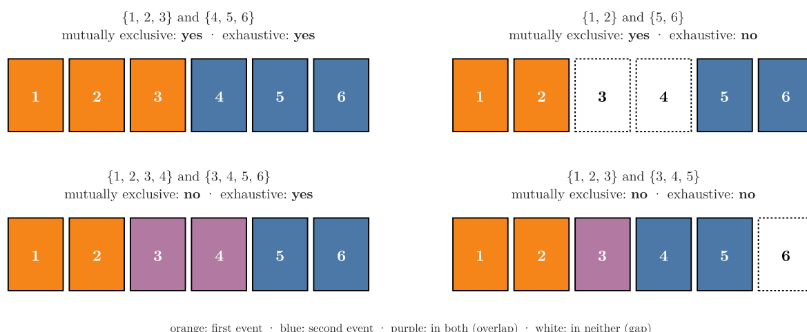
Figure 7: The four rows of the table on die faces. Purple faces belong to both events (an overlap); white faces belong to neither (a gap).
