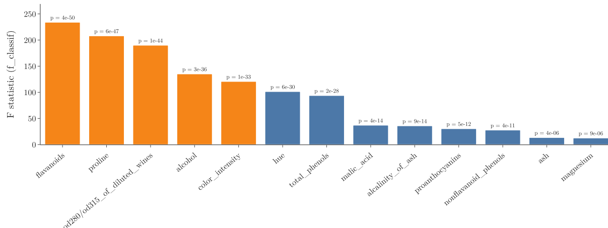
Figure 6: One ANOVA F test per feature of the wine dataset ( f_classif ), with each p-value above its bar. SelectKBest(k = 5) keeps the five features with the largest F (orange).
