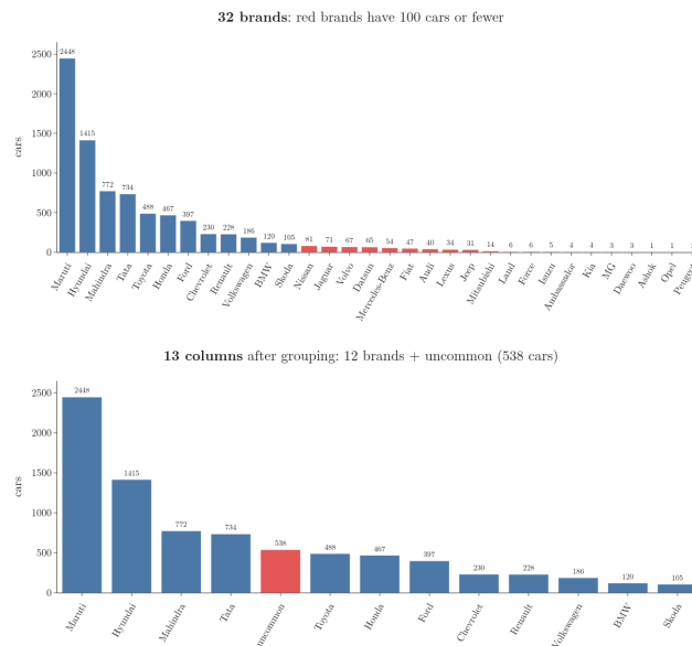
Figure 9: The 32 brands of the car data, then the 13 columns left after the 20 brands with 100 cars or fewer (red) are replaced by uncommon , which holds 538 cars.
