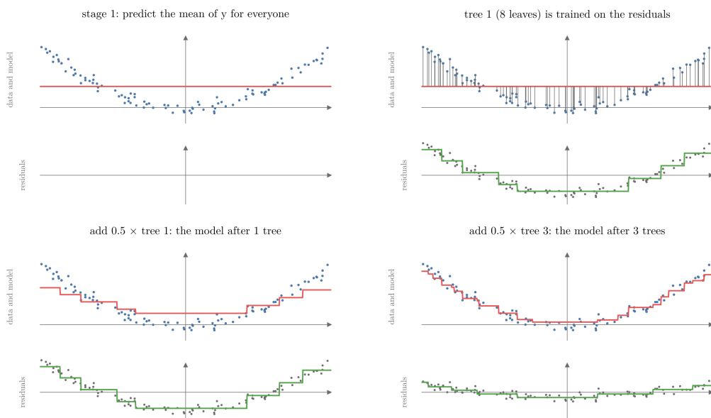
Figure 7: Gradient boosting on the curve, learning rate 0.5: residuals of the current model (grey), the tree trained on them (green), and the model after adding half of it (red)
