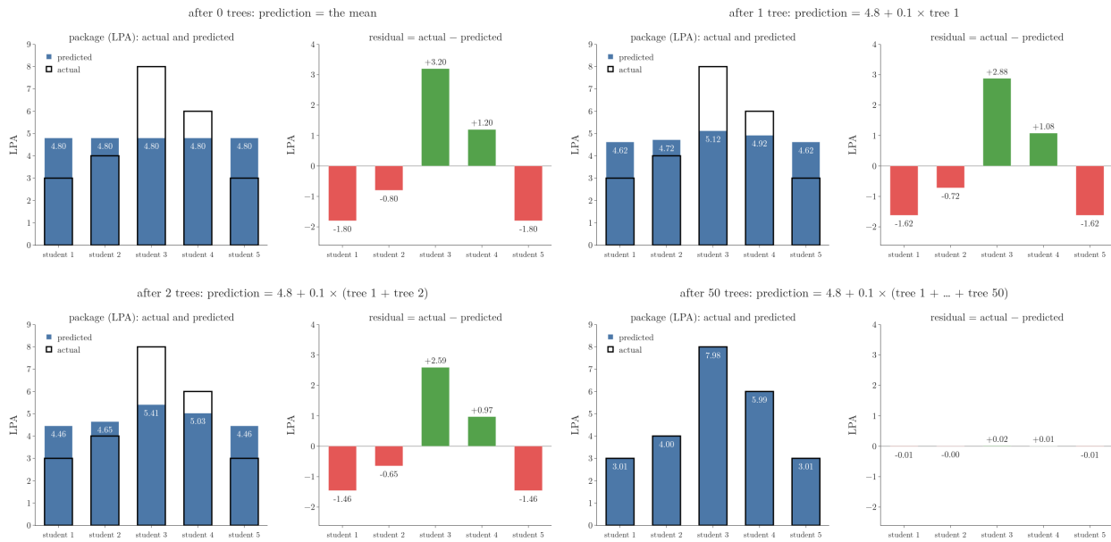
Figure 5: Gradient boosting on the five students, learning rate 0.1. Left: actual package (outline) and the model's prediction (blue bar). Right: the residuals the next tree is trained on
