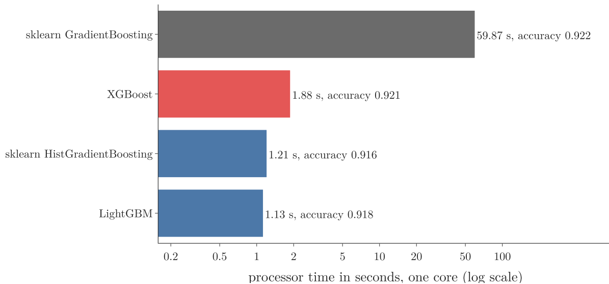
Figure 5: Processor time on 10,000 observations and 200 features, 100 trees of depth 3 in every library, one core each (log scale)
