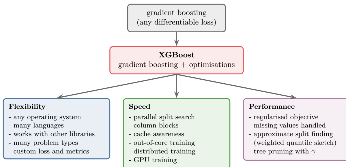
Figure 1: XGBoost: gradient boosting plus optimisations in three areas
