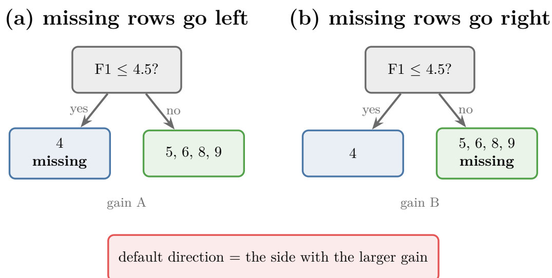
Figure 8: Sparsity-aware split finding: observations with a missing value are tried on each side; the side with the larger gain becomes the default direction
