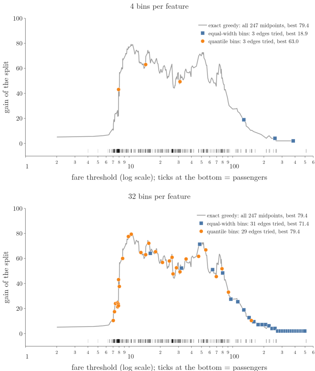
Figure 9: Exact greedy versus approximate split finding on the 891 Titanic fares, target Survived. Grey: the gain of the first XGBoost tree (log loss, \lambda = 1 ) at each of the 247 exact midpoints. Orange: quantile bin edges; blue: equal-width bin edges; 4 to 64 bins per feature
