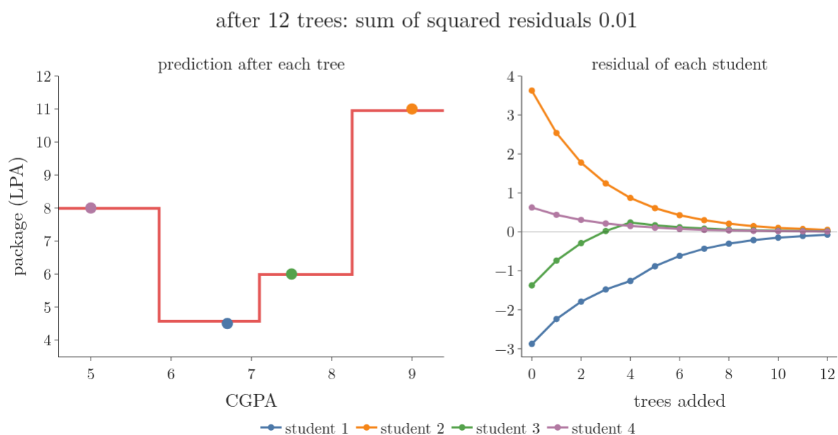
Figure 7: The boosting loop on the four students ( \eta = 0.3 , \lambda = 0 , depth 2). Left: the prediction after each tree. Right: each student's residual, tree after tree
