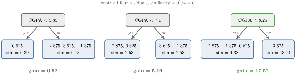
Figure 4: The three candidate root splits, with each leaf's residuals and similarity score; \text{CGPA} < 8.25 has by far the largest gain
