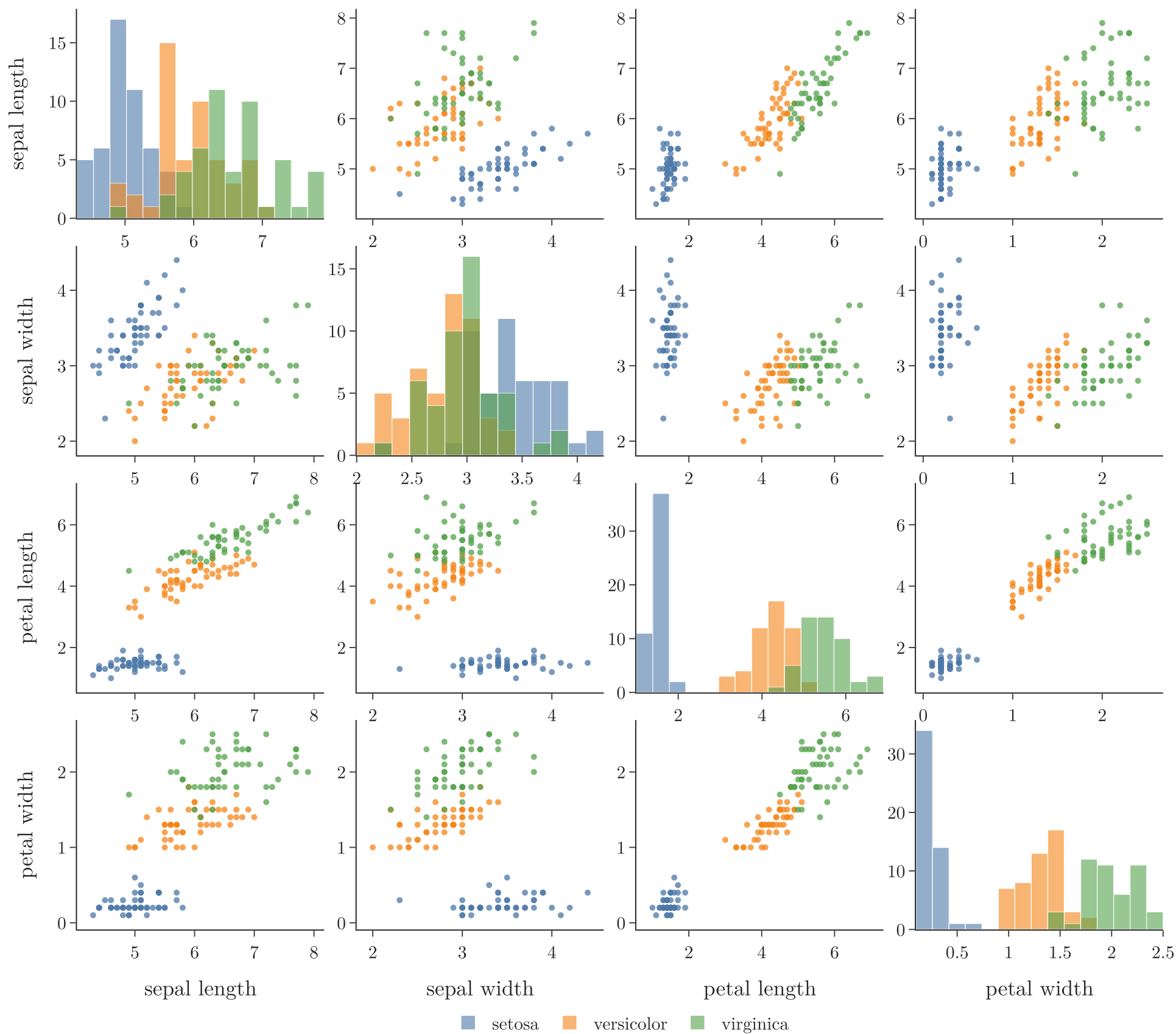
Iris: every pair of measurements
