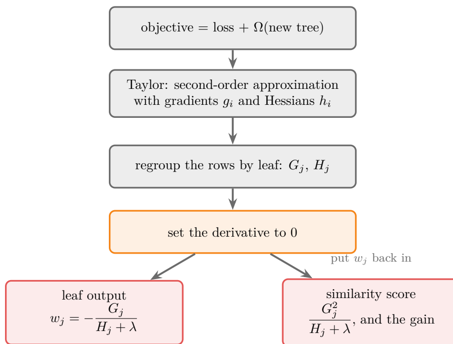
Figure 1: The derivation in five steps: from the objective to the leaf output, the similarity score and the gain
