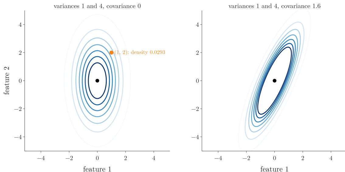
Figure 7: Contours of two-dimensional normal components with variances 1 and 4. Left: no covariance, ellipses along the axes; the example point (1, 2) has density 0.0293. Right: covariance 1.6, tilted ellipses.
