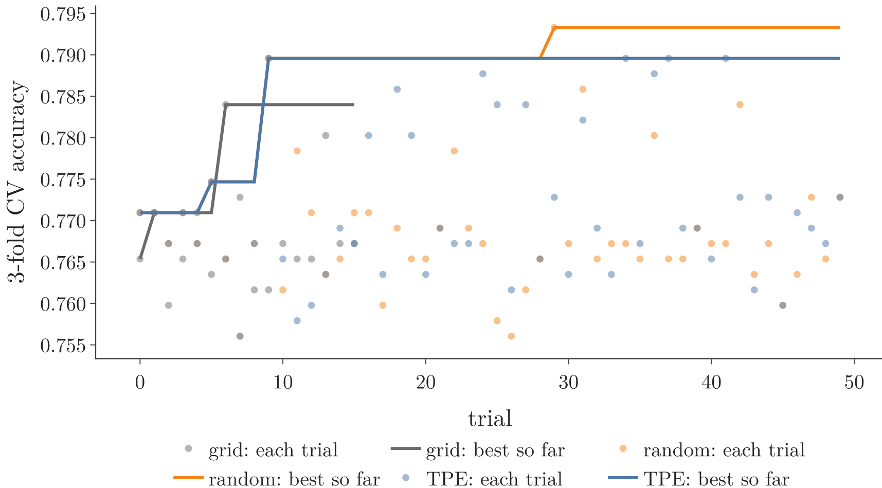
Optimisation history: grid, random and TPE
