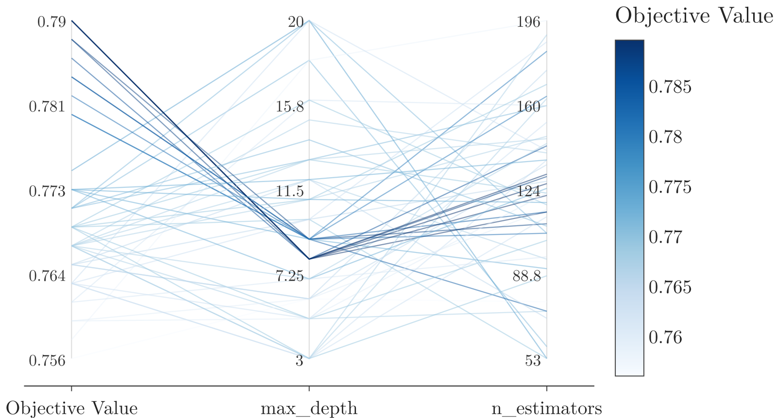
Parallel coordinates of the TPE study
