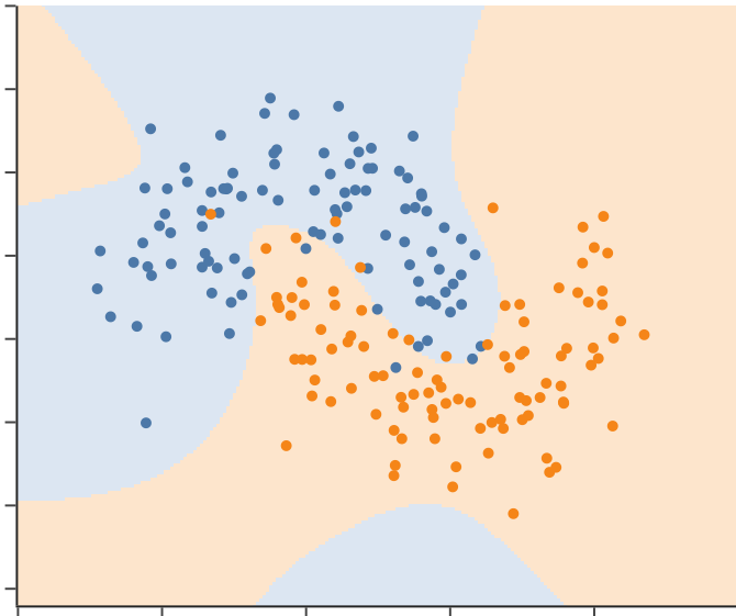
degree 4 (14 columns): CV accuracy 0.935
