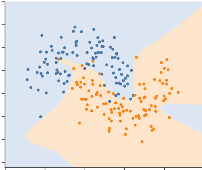
degree 10 (65 columns): CV accuracy 0.900
