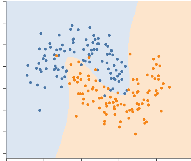
degree 3 (9 columns): CV accuracy 0.920
