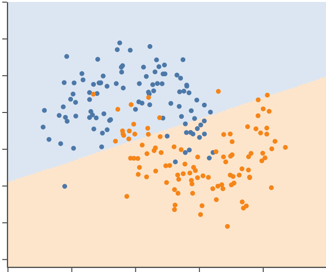
degree 1 (2 columns): CV accuracy 0.830
