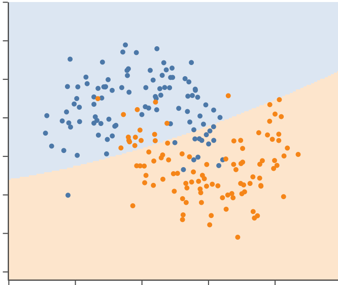
degree 2 (5 columns): CV accuracy 0.835
