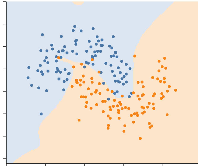
degree 25 (350 columns): CV accuracy 0.905
