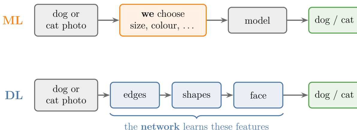
Figure 1: Who finds the features. In ML we choose them (size, colour); in DL the layers learn them, from edges to shapes to a face
