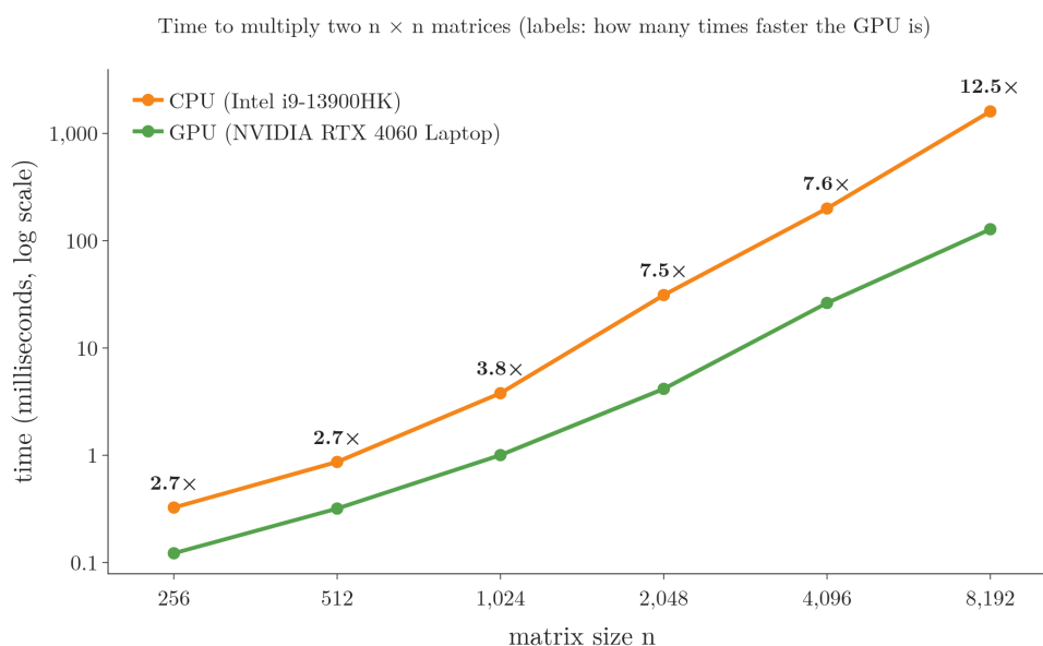
Figure 7: Time to multiply two n by n matrices on a laptop CPU and a laptop GPU, with TensorFlow. Labels: how many times faster the GPU is.
