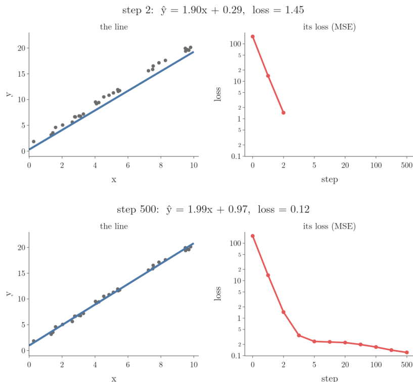
Figure 2: Gradient descent on the 30 points of Figure 6 that follow y = 2x + 1 : the line moves (left) while its MSE loss falls (right)
