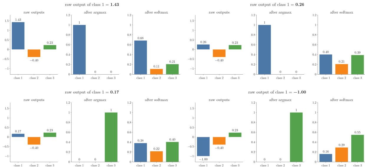
Figure 10: Three raw outputs (left), after argmax (middle) and after softmax (right), while the raw output of class 1 slides from 1.43 down to -1 . Idea after StatQuest, “Neural Networks Part 5: ArgMax and SoftMax”
