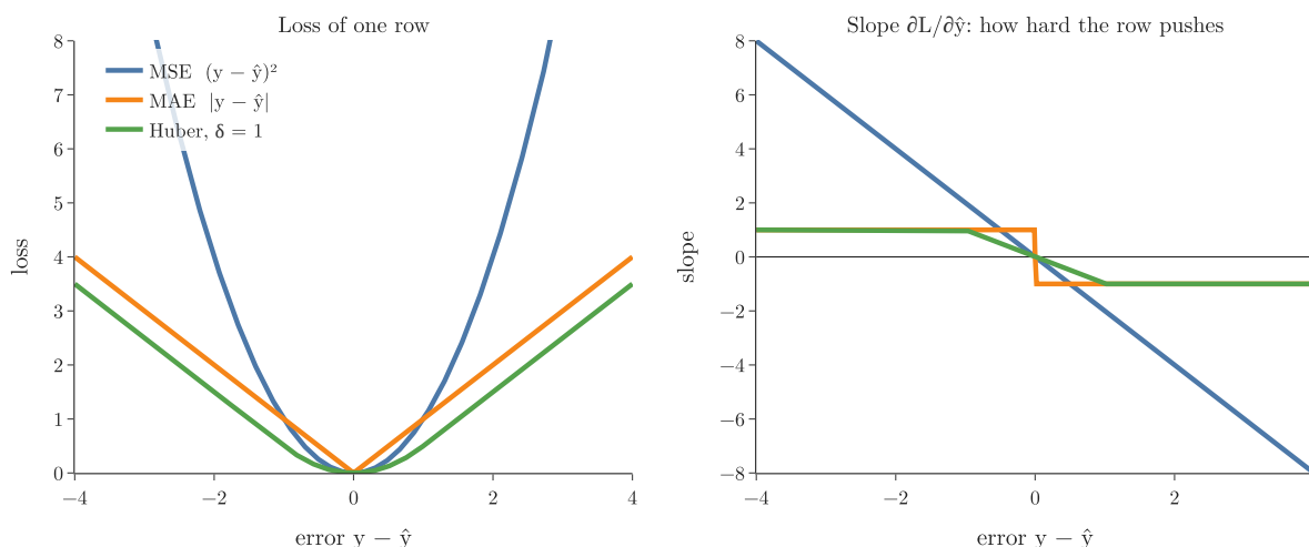
Figure 4: Left: the loss of one observation against its error. Right: its slope, which sets how hard the observation pushes the weights
