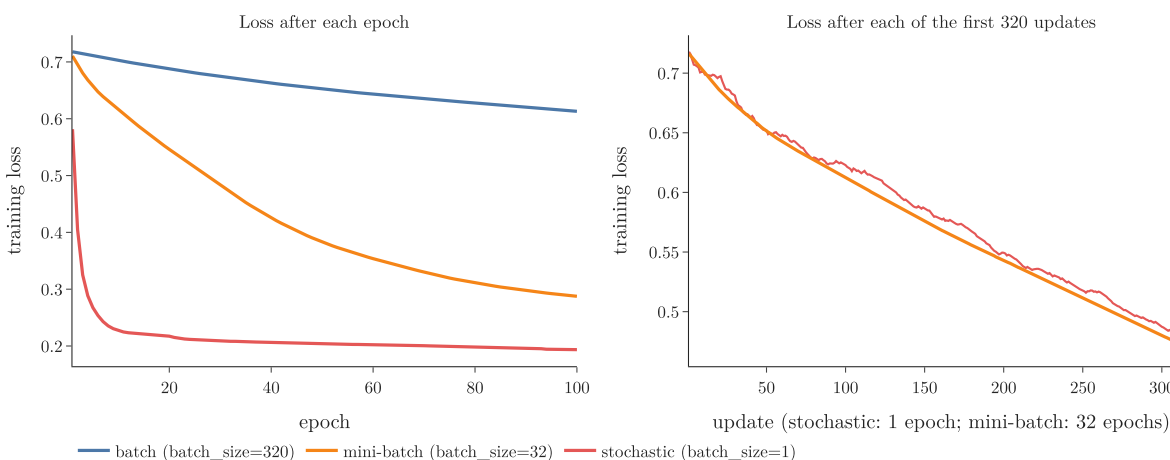
Figure 8: Left: training loss per epoch over 100 epochs. Right: loss on all 320 training observations after each single update
