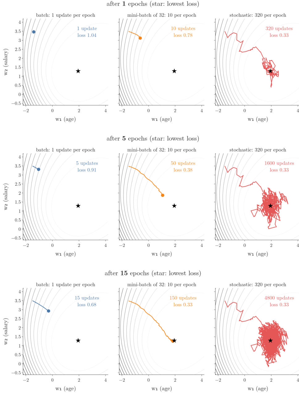
Figure 7: The three variants as paths on one loss surface, epoch by epoch. The model is a single sigmoid neuron on the first 320 observations, with one weight for age and one for salary; grey lines are contours of the loss and the star is its lowest point. All three start at the same point with learning rate 0.3
