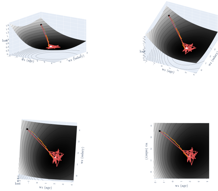
Figure 6: The loss surface of the one-neuron model over the age weight w_1 and the salary weight w_2 : a smooth bowl. The camera tilts from a side view to the top view; the black lines join points at the same height. The coloured paths are those of Figure 7 (blue: batch, orange: mini-batch, red: stochastic); black dot: start; white diamond: lowest point
