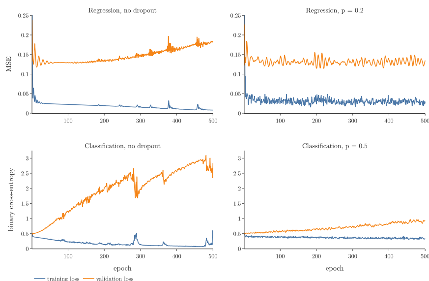
Figure 2: Training and validation loss. Top: regression without dropout and with p = 0.2 . Bottom: classification without dropout and with p = 0.5 .
