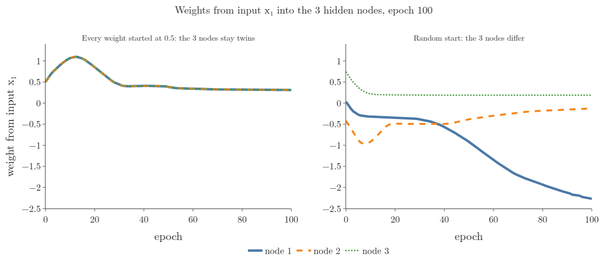
Figure 4: The weights from input x_1 into the 3 ReLU hidden nodes during 100 epochs. Left: every weight and bias started at 0.5. Right: Keras' random start.
