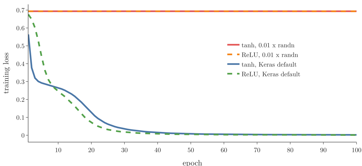
Figure 5: Training loss of the four-layer network with plain SGD. Started from 0.01 \times standard normal, tanh and ReLU stay at 0.693 for 100 epochs. Started from Keras’ default, both fall to near 0
