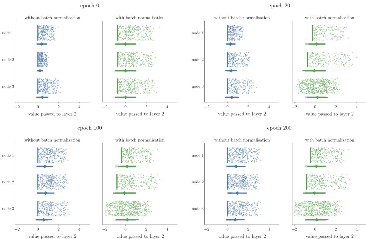
Figure 3: What the second hidden layer receives during training, with and without batch normalisation. Each dot is one observation’s value at one node of the first hidden layer; the bar is the mean plus and minus one standard deviation, the grey bar the same at the start
