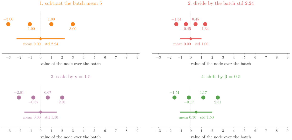
Figure 4: The batch z = 2, 4, 6, 8 of one node through batch normalisation: subtract the batch mean, divide by the batch standard deviation, scale by \gamma = 1.5 , shift by \beta = 0.5 . The bar is the mean plus and minus one standard deviation
