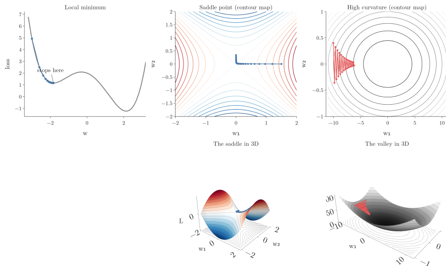
Figure 3: Plain gradient descent on the three obstacles. Left: from w = -3 it stops in the small dip (learning rate 0.05). Middle: on the saddle L = w_1^2 - w_2^2 , starting almost on the ridge, its steps shrink to almost nothing near the flat centre before it slides off. Right: on the narrow valley (learning rate 0.019) it zigzags across the steep sides. Bottom: the saddle and the valley as 3D surfaces, same contour levels and same paths (blue on the saddle, red on the valley); the colours mark height, red high and blue low on the saddle, dark low and light high on the valley.
