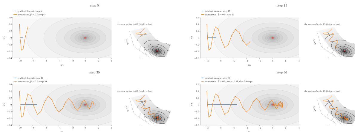
Figure 1: Plain gradient descent and momentum along a narrow valley, same learning rate 0.01. Gradient descent drops to the valley floor and crawls along it; momentum builds speed along the valley
