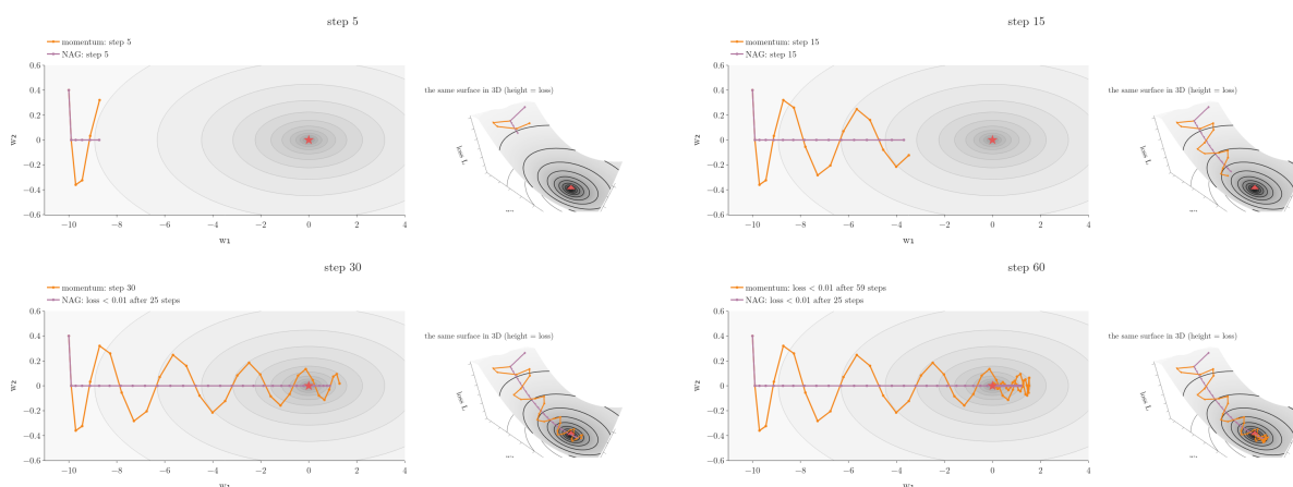
Figure 1: Momentum and NAG along the same narrow valley, both with learning rate 0.01 and \beta = 0.9 . Momentum swings across the valley and past the minimum; NAG's swings are much smaller
