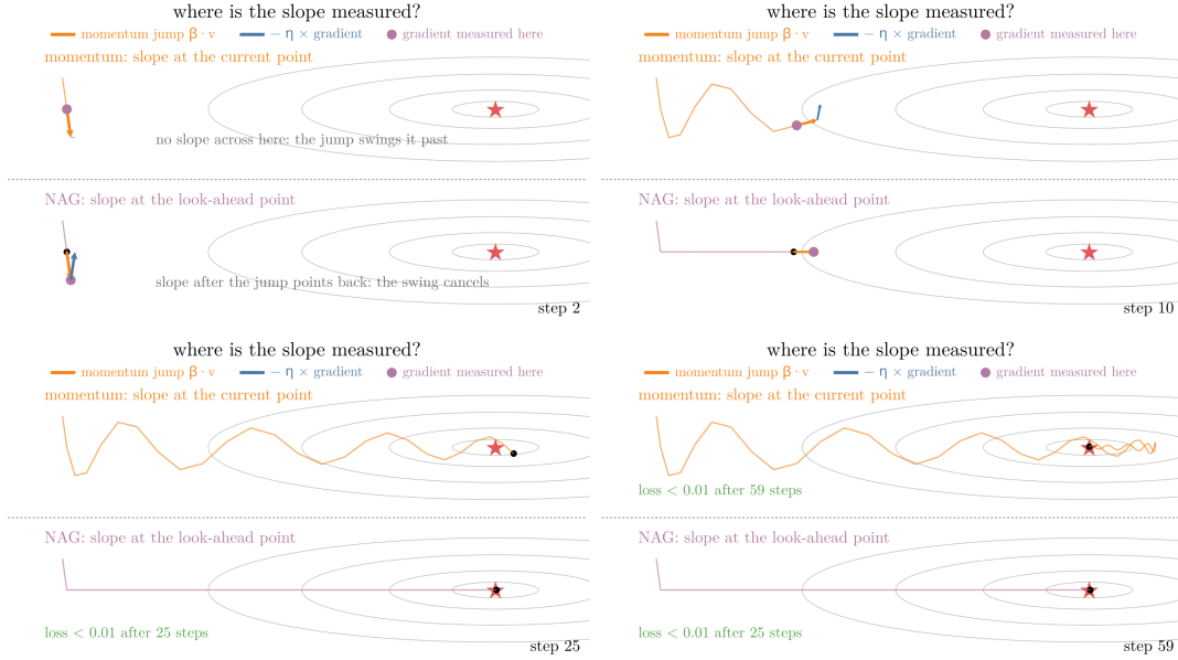
Figure 4: Momentum (top) and NAG (bottom) step by step on the valley of Figure 1. Orange: the jump \beta v_{t-1} ; blue: -\eta times the gradient; purple dot: where the gradient is measured. Momentum measures at the current point, NAG at the look-ahead point
