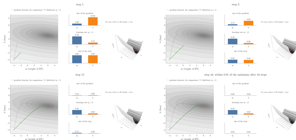
Figure 4: AdaGrad, \eta = 2 , on the students data, step by step. Left: its path (green) beside gradient descent's (grey). Right, for m (blue) and b (orange): the size of the gradient, the learning rate \eta/\sqrt{v} and the size of the update
