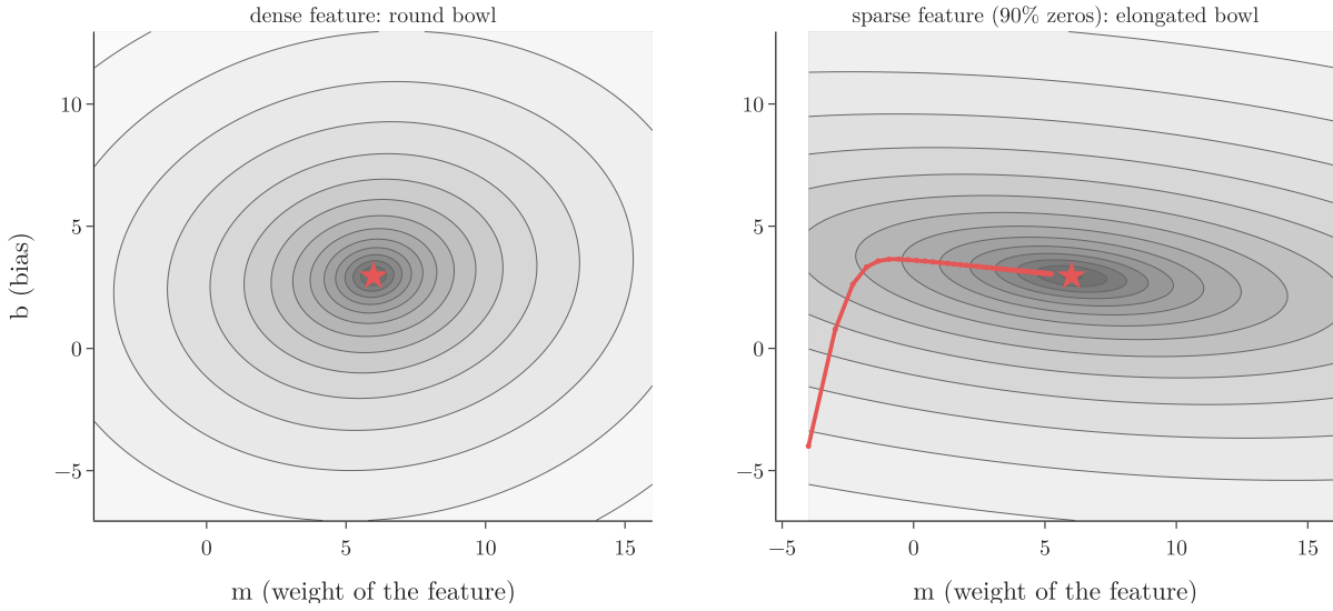
Figure 3: The loss over (m, b) . Left: with a dense feature (no zeros) the contours are nearly round. Right: with the sparse IIT feature the bowl is stretched along m . Red: gradient descent ( \eta = 0.3 ) from (-4, -4) , as drawn on the surface in Figure 2; star: the minimum
