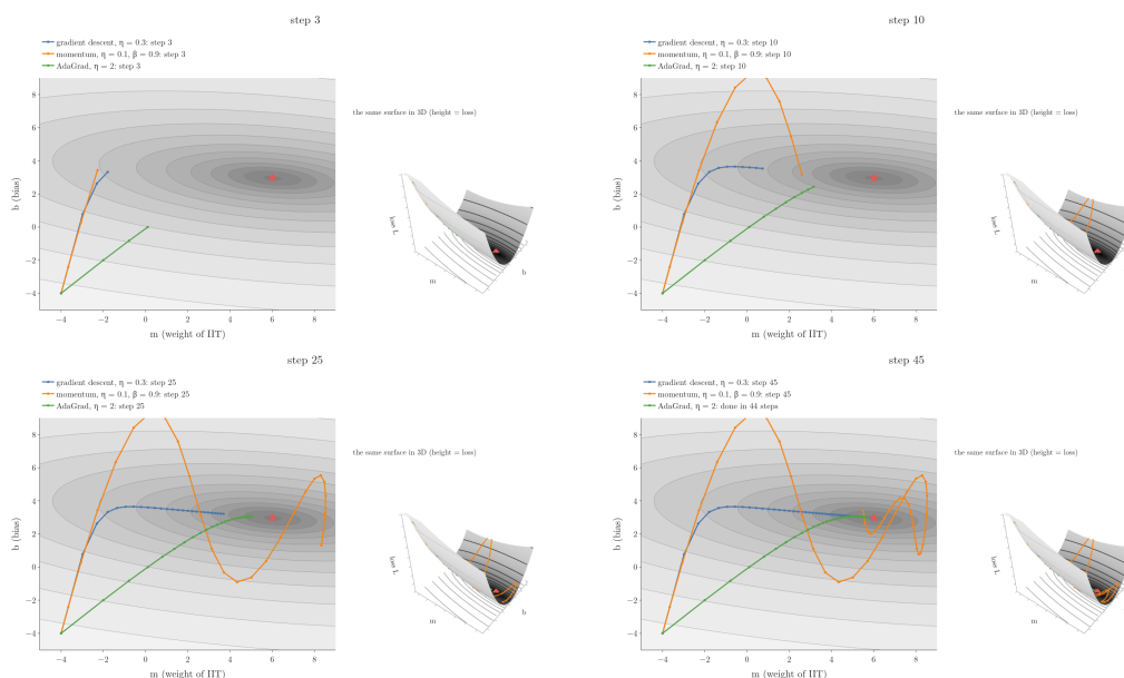
Figure 1: Gradient descent, momentum and AdaGrad on a loss stretched by a sparse feature. Gradient descent first moves along b , then crawls along m ; momentum also shoots along b first, then swings in wide loops; AdaGrad heads for the minimum
