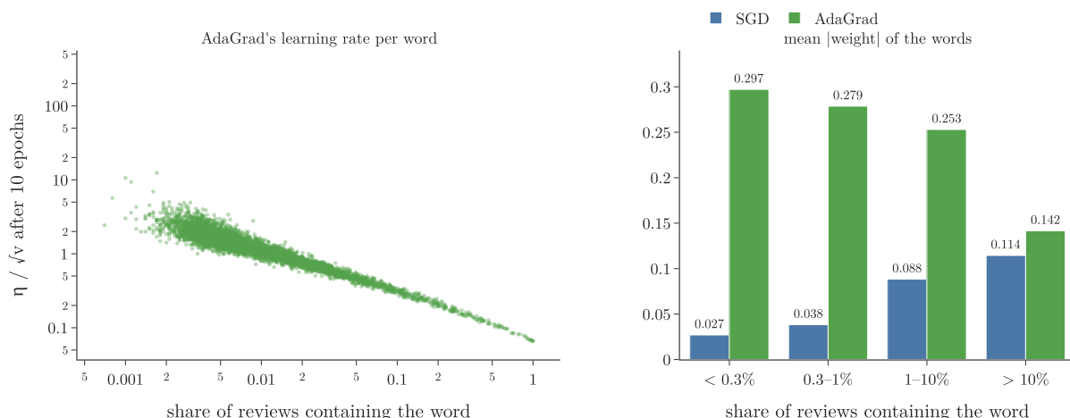
Figure 5: IMDB, 5,000 words. Left: AdaGrad's learning rate for each word after 10 epochs against the share of reviews containing the word; the rarer the word, the larger its learning rate. Right: mean size of the learned weights per frequency band; with SGD the rare words barely move
