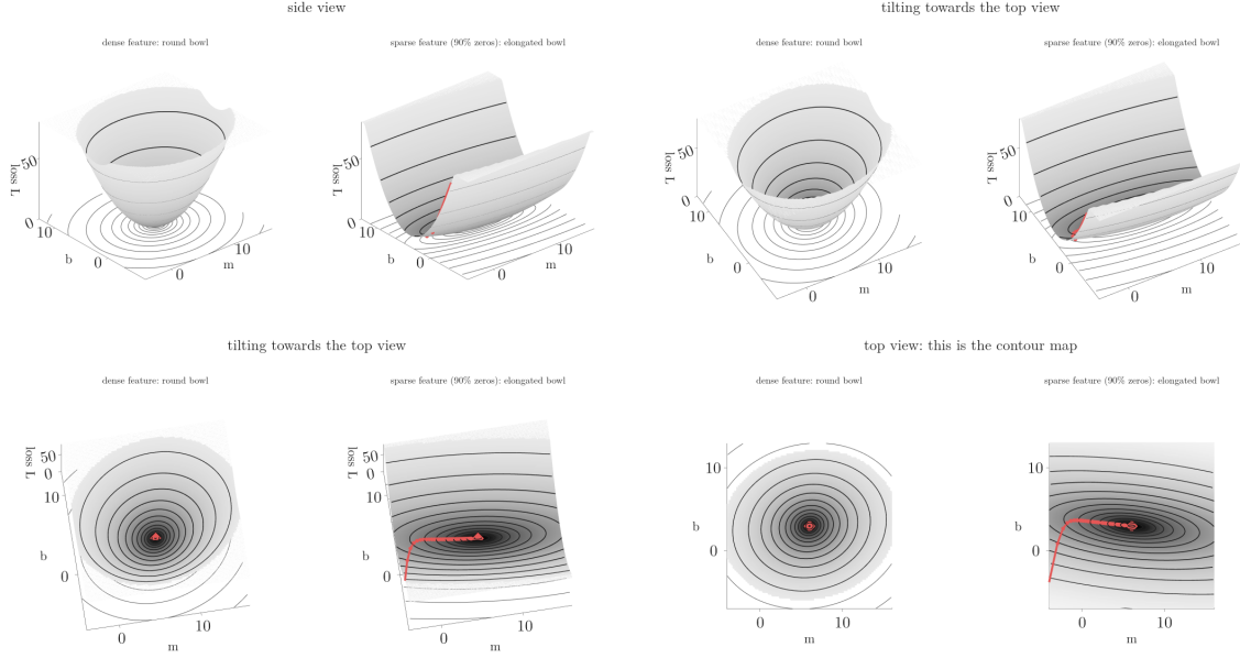
Figure 2: The two losses as surfaces, tilting from the side view to the top view. Left: a dense feature. Right: the sparse IIT feature, with gradient descent ( \eta = 0.3 ) from (-4, -4) in red. Height is the loss L , cut flat at 80: the walls go higher than drawn. Thin lines join points of equal height, on the surface and dropped to the floor, each about 1.6 times the one inside it; the diamond is the minimum
