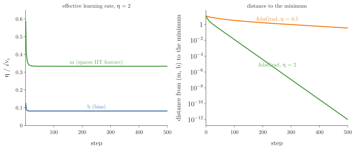
Figure 6: AdaGrad on the students data. Left: the effective learning rates of m and b with \eta = 2 fall in the first steps and never rise again. Right: distance to the minimum; with \eta = 2 AdaGrad converges, with \eta = 0.5 it is still 0.35 away after 500 steps
