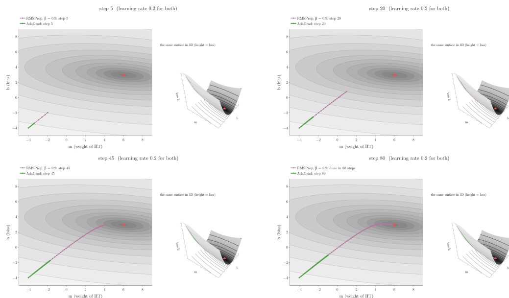
Figure 1: AdaGrad and RMSProp with the same learning rate 0.2 on the elongated bowl of a sparse feature. AdaGrad's steps keep shrinking and it crawls; RMSProp keeps moving and reaches the minimum
