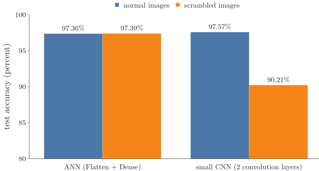
Figure 6: Mean test accuracy on normal and scrambled MNIST. The vertical axis starts at 80 percent, not 0, so that the gap is visible. The ANN does not notice the scrambling; the CNN loses 7 points, because it was using which pixels are neighbours
