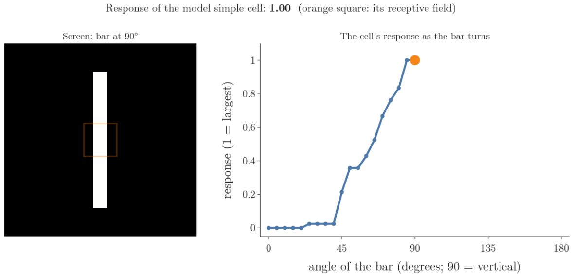
Figure 3: The Hubel and Wiesel experiment, replayed with a model cell. Left: the screen, with a bar of light rotating from horizontal (0°) to vertical (90°) and back; the orange square is the cell's receptive field. Right: the cell's response at each angle.
