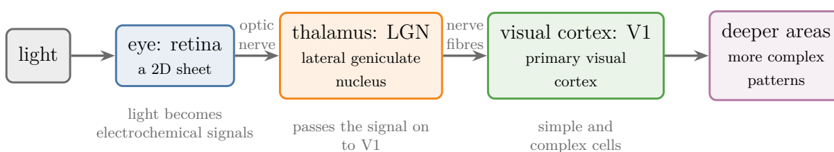
Figure 2: The path of visual information: retina, optic nerve, lateral geniculate nucleus (in the thalamus), primary visual cortex V1, deeper areas
