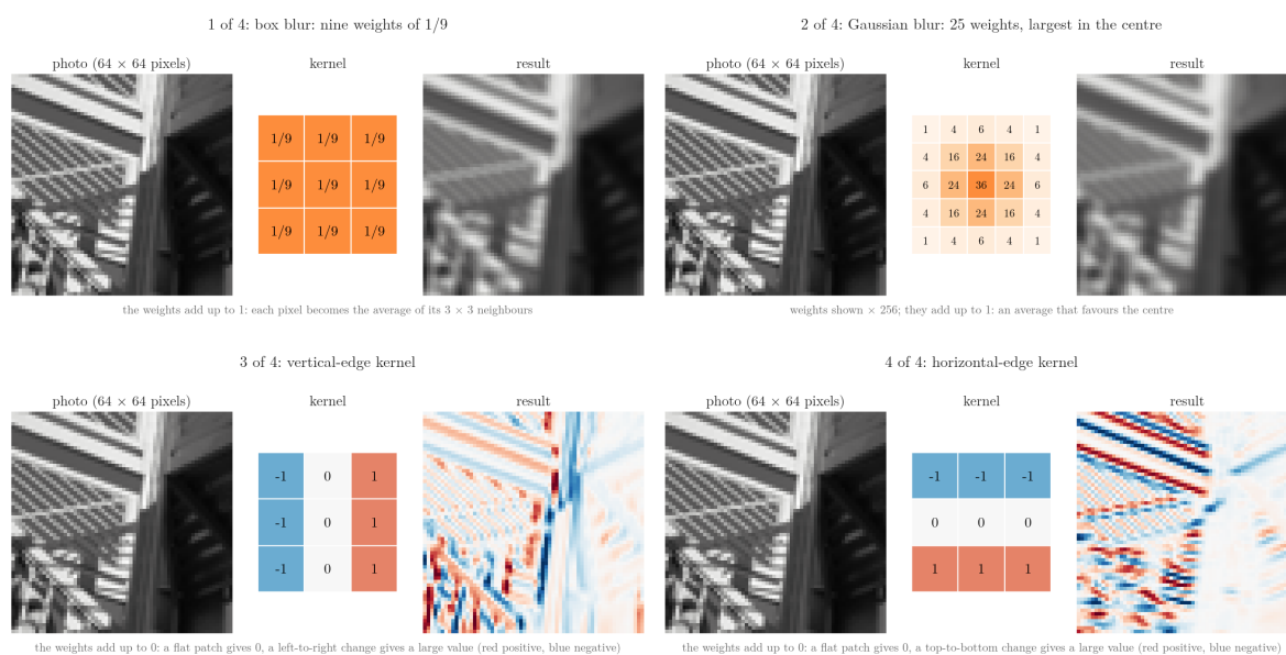
Figure 4: One 64 \times 64 piece of the photo convolved with four kernels, one per frame: box blur, Gaussian blur, vertical-edge kernel, horizontal-edge kernel. Each frame shows the kernel and its result. Sequence of kernels after 3Blue1Brown, “But what is a convolution?”
