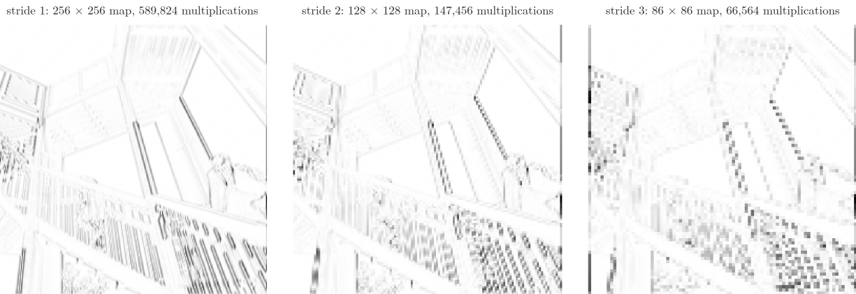
Figure 6: One vertical-edge filter on a 256 \times 256 photo, with padding 1, at strides 1, 2 and 3. Darker means a stronger edge. The titles give the size of the feature map and the multiplications needed.
