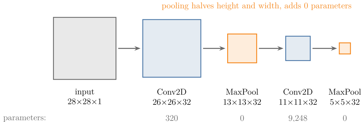
Figure 4: The output of each layer of the model above, drawn to scale (side = height of the map), with its parameter count.
