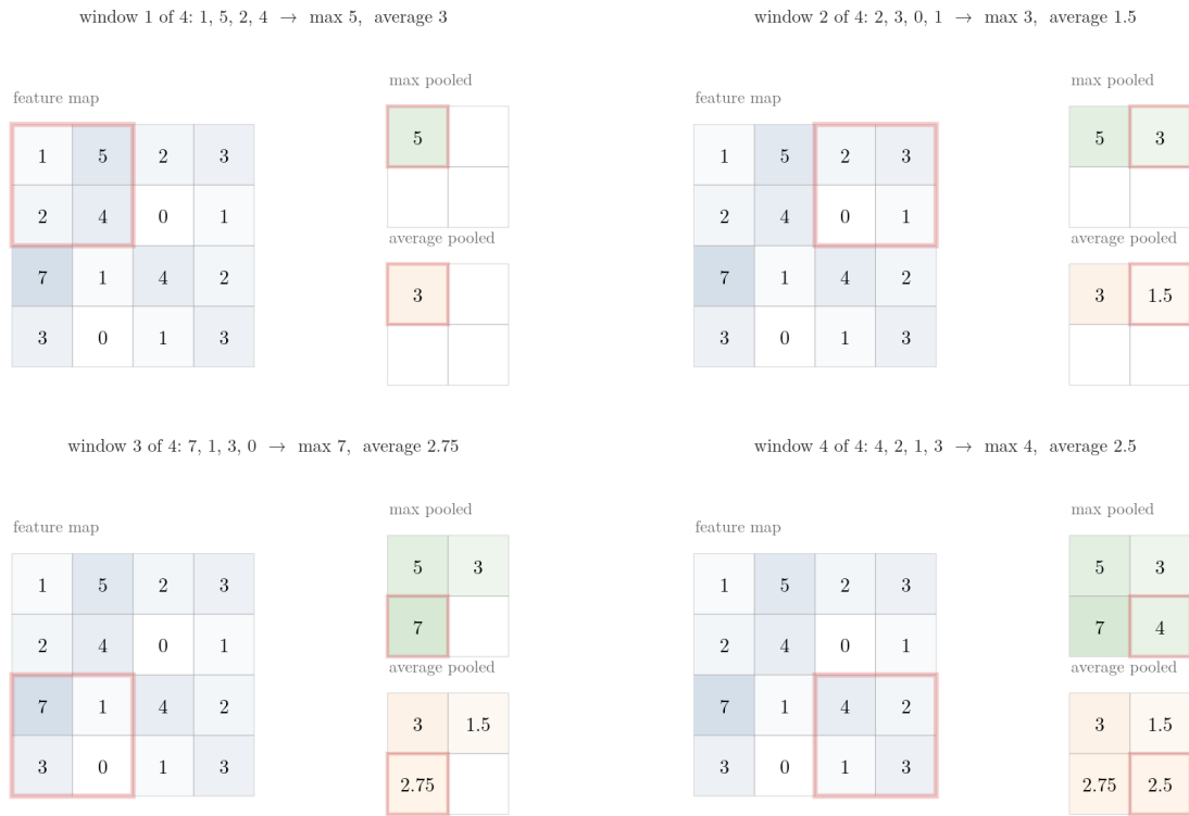
Figure 8: The map of section 4.3 pooled two ways at once. The same 2 \times 2 window (red) fills the max-pooled map (green) and the average-pooled map (orange)
