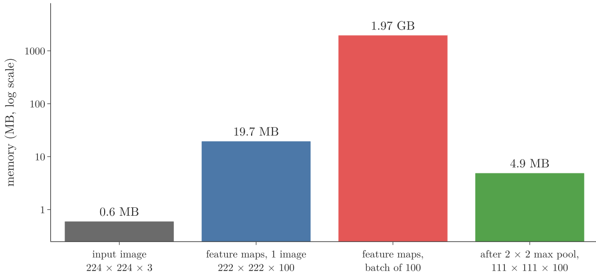
Figure 2: Memory of one input image, of the feature maps one convolution layer of 100 filters makes from it, of those maps for a batch of 100 images, and of one image’s maps after 2 \times 2 max pooling (section 7.1). Log scale; 4 bytes per number.
