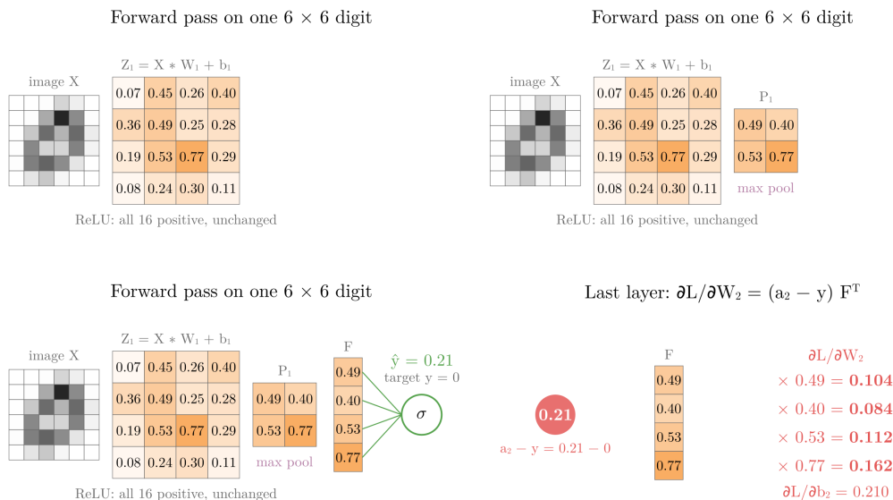
Figure 3: The Notebook's first image, a 0 shrunk to 6 \times 6 , through the small CNN with the Notebook's starting weights. The 3 \times 3 filter slides over X to fill Z_1 ; ReLU changes nothing here, since all 16 values are positive; each 2 \times 2 window sends its maximum to P_1 ; flatten gives F and the sigmoid gives \hat{y} = 0.21 . Then the error a_2 - y = 0.21 multiplies each value of F to give \partial L / \partial W_2 (section 6.2)
