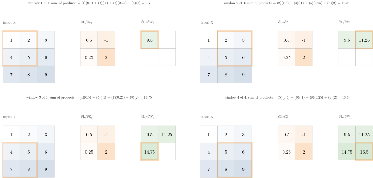
Figure 7: The example above, one window per frame: the 2 \times 2 gradient \partial L / \partial Z_1 (orange) slides over the 3 \times 3 input X like a filter, and each stop fills one cell of \partial L / \partial W_1 (green)
