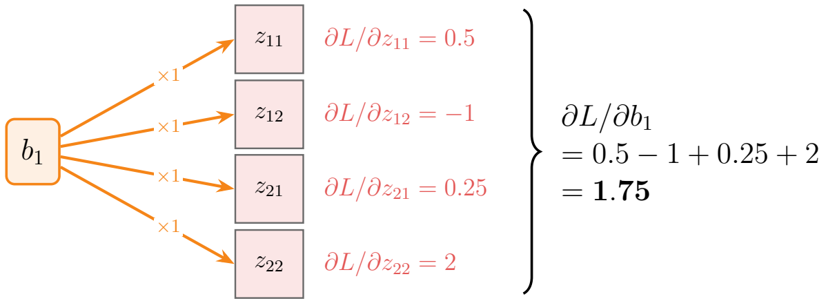
Figure 6: The bias reaches the loss along four paths, one through each value of Z_1 , each with local derivative 1; the chain rule adds the four gradients.
