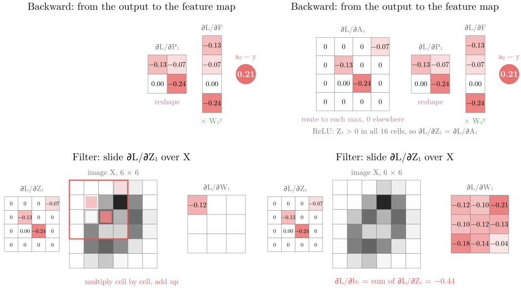
Figure 8: The whole backward pass on the 6 \times 6 digit of the part 1 Note, with the same weights. The error a_2 - y = 0.21 is multiplied by W_2^T , reshaped to 2 \times 2 , and routed to the maximum of each pooling window of A_1 . ReLU passes everything here, because all 16 values of Z_1 are positive. Then \partial L / \partial Z_1 slides over X like a filter: each position fills one cell of \partial L / \partial W_1
