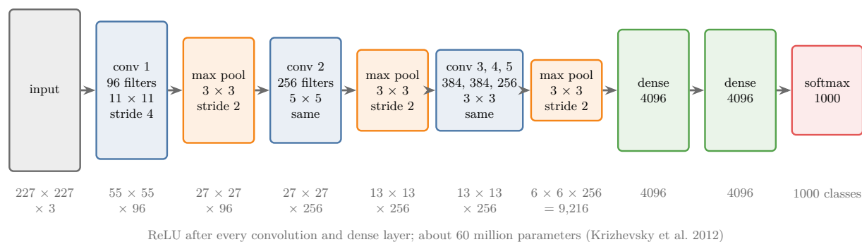
Figure 4: AlexNet: five convolution layers (blue), three max-pooling layers (orange), two dense layers of 4,096 nodes (green) and a third dense layer, the 1,000-way softmax output (red; a layer giving one probability for each of the 1,000 classes). Under each layer: the size of its output
