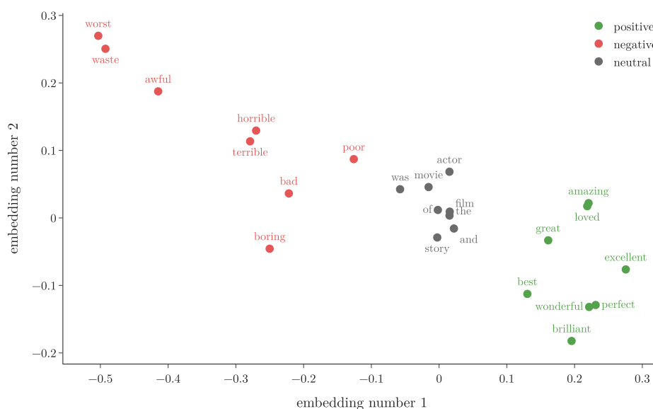
Figure 6: The learned 2-number vectors of a few IMDB words after training. Positive words (green) and negative words (red) end up on opposite sides; frequent neutral words (grey) sit between them
