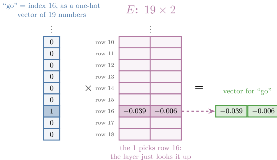
Figure 5: The embedding layer as a lookup: the one-hot vector of “go” (index 16, drawn standing up to save space; in the product it is a row of 19 numbers) times E keeps row 16 of E , which becomes the word's dense vector
