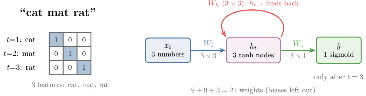
Figure 2: Left: the review “cat mat rat” as a 3 \times 3 table, one row per time step and one column per feature. Right: the network, with the shape of each weight matrix. W_h feeds the hidden state back into the same layer
