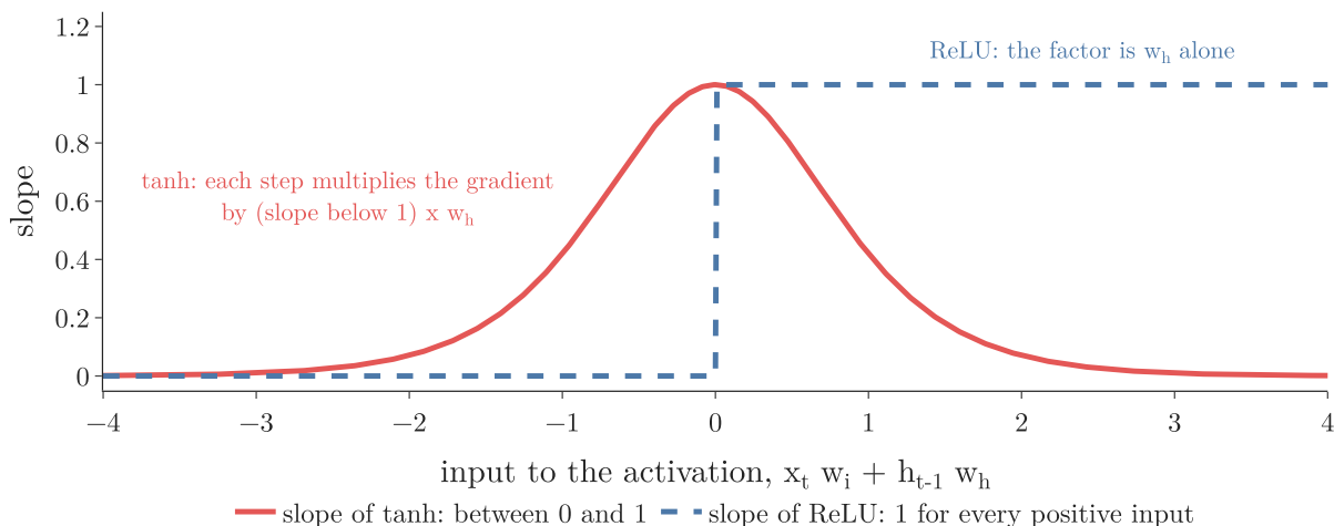
Figure 6: The slope of the activation, which multiplies w_h at every backward step. tanh's slope (red) is 1 only at 0 and smaller everywhere else, so each step shrinks the gradient. ReLU's slope (blue) is exactly 1 for every positive input, so the factor is w_h alone
